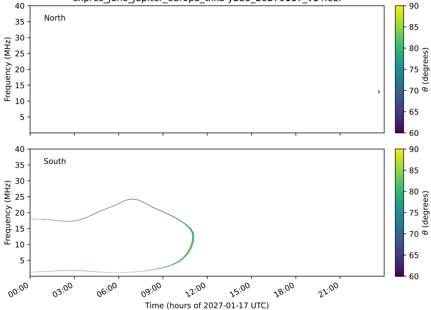
expres_juno_jupiter_europa_txka-y235_20270117_v14.cdf
