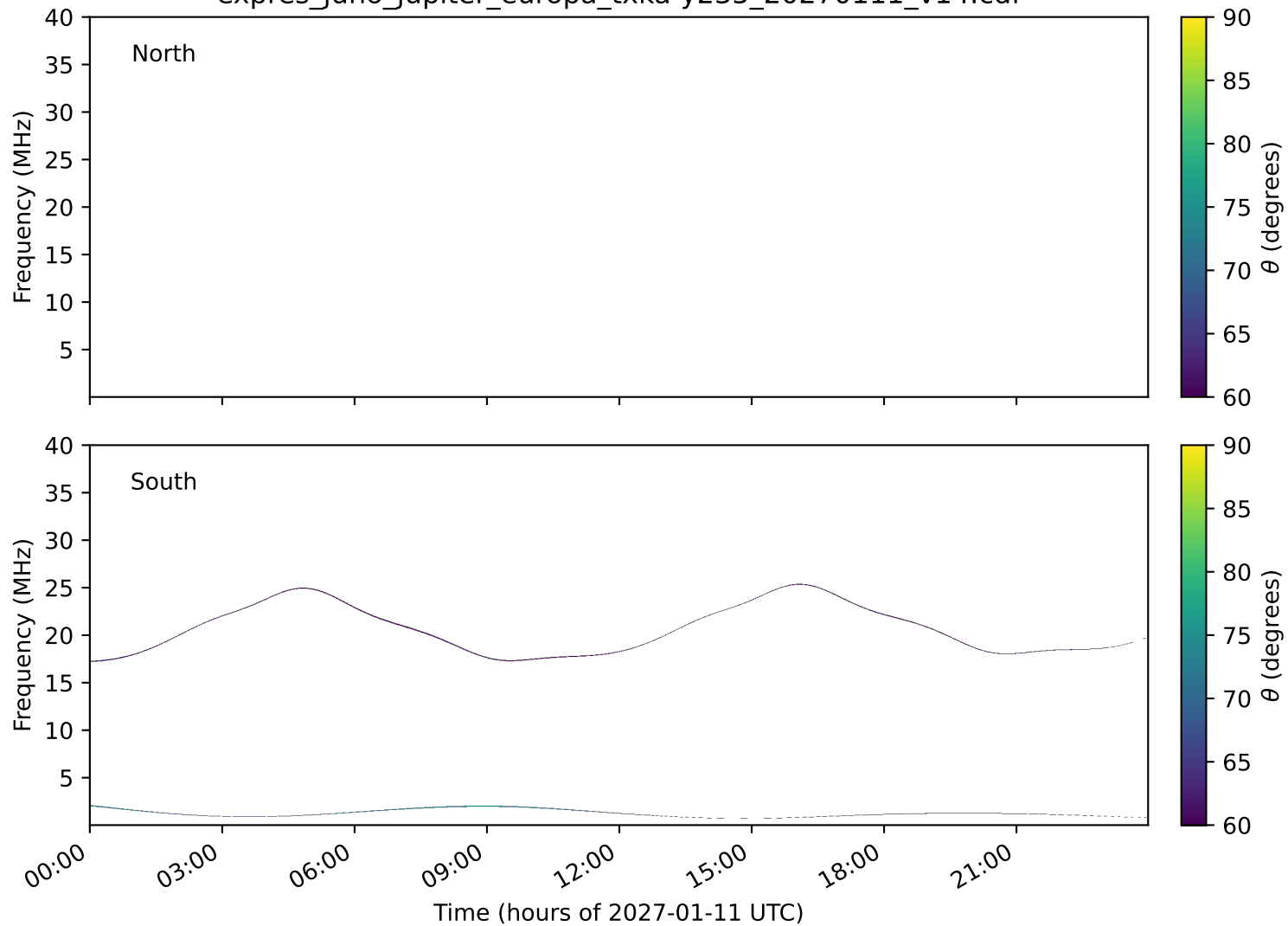
expres_juno_jupiter_europa_txka-y235_20270111_v14.cdf
