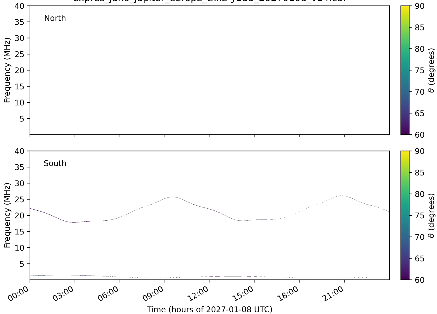
expres_juno_jupiter_europa_txka-y235_20270108_v14.cdf
