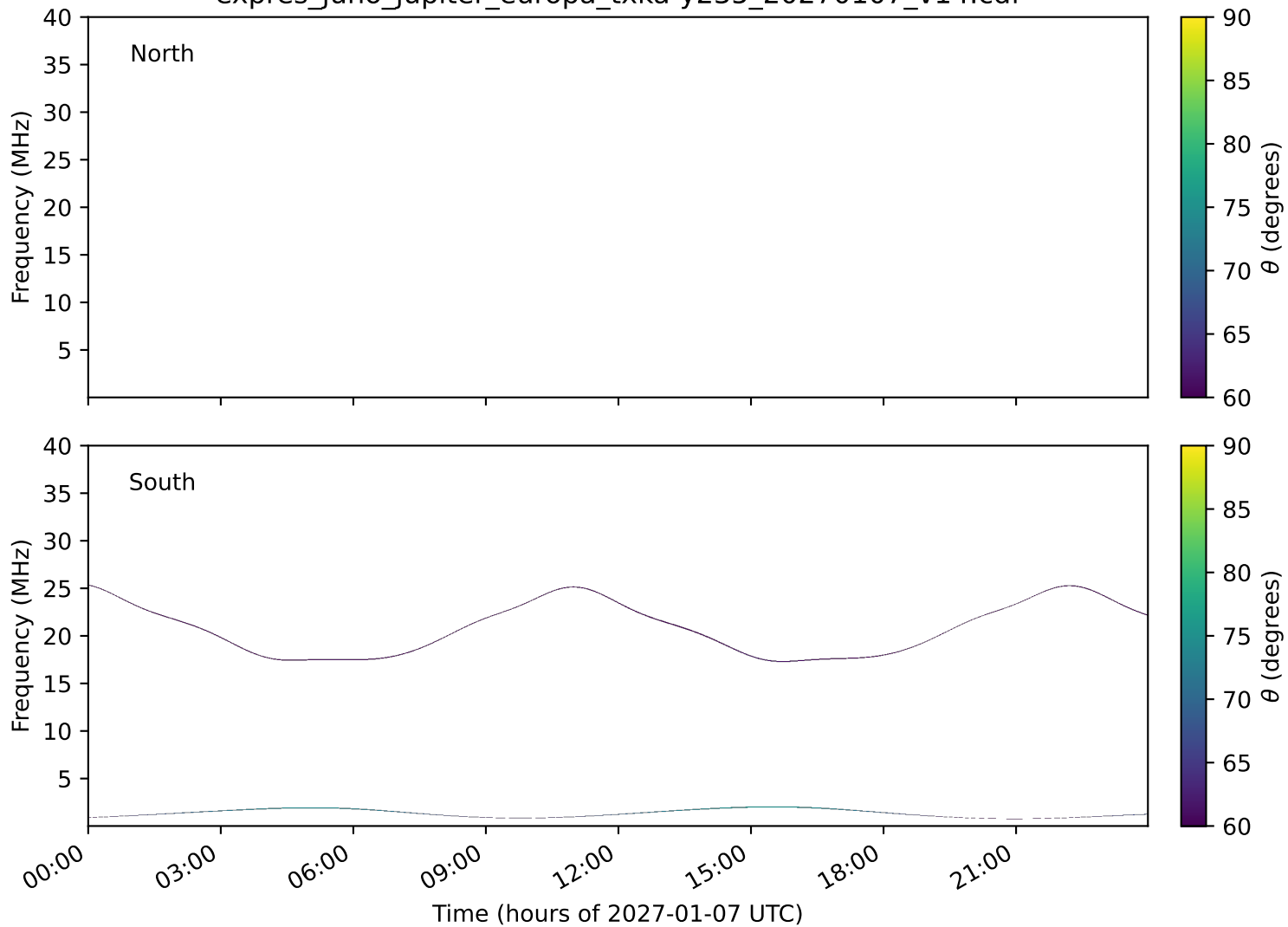
expres_juno_jupiter_europa_txka-y235_20270107_v14.cdf
