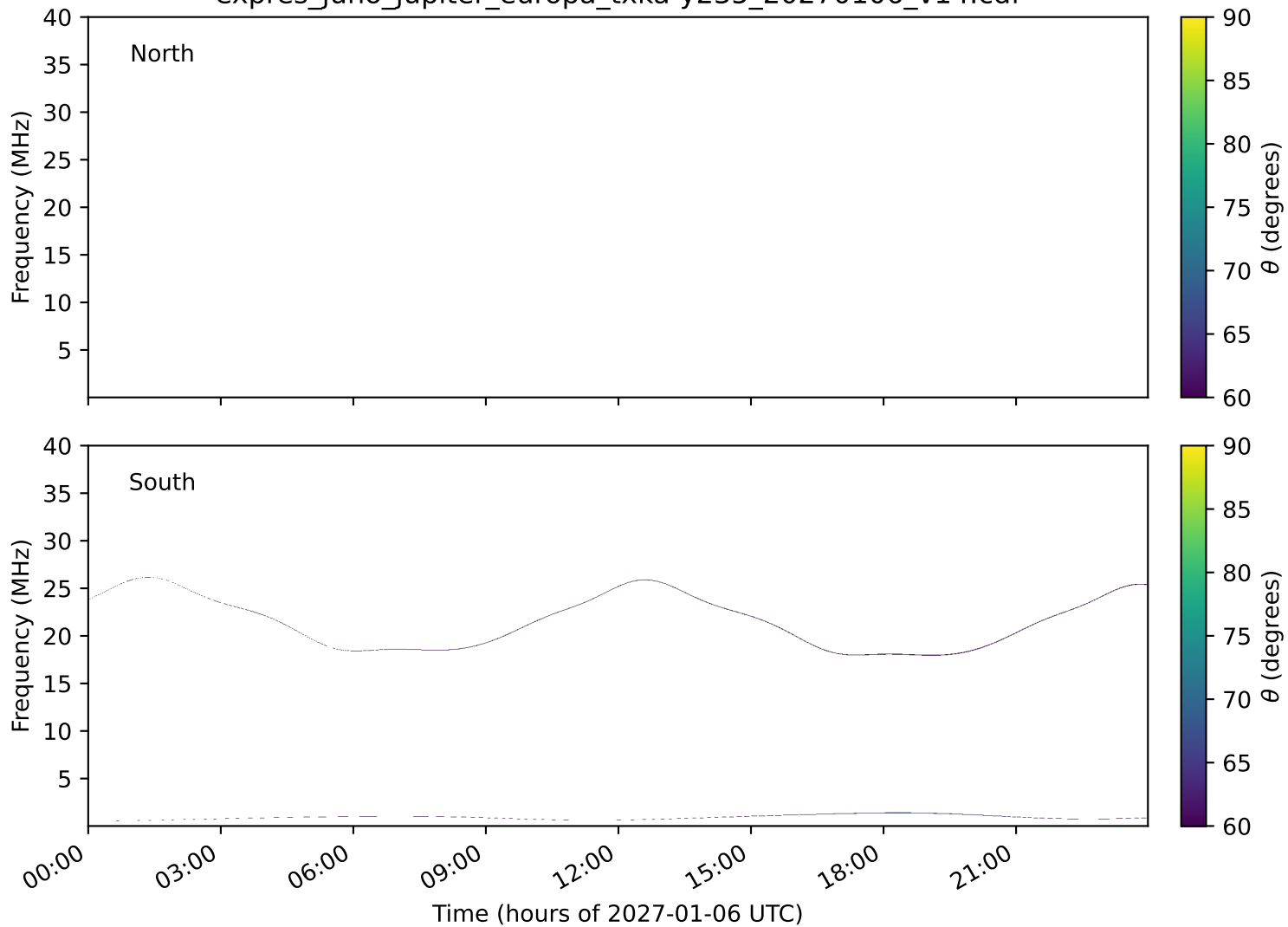
expres_juno_jupiter_europa_txka-y235_20270106_v14.cdf
