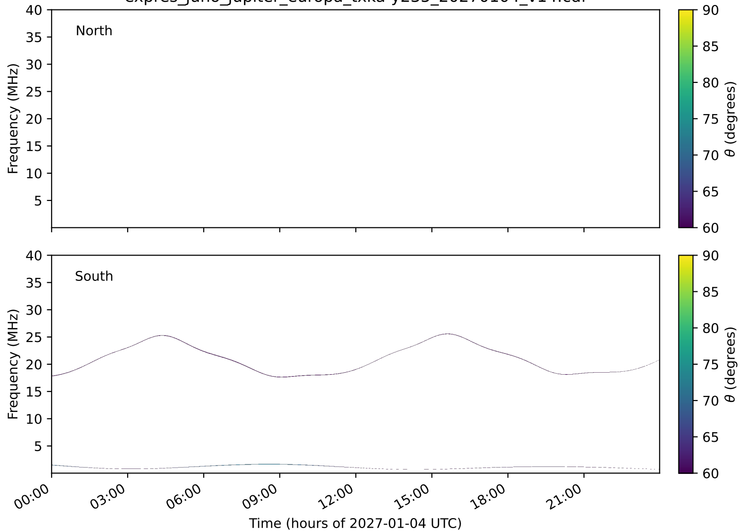
expres_juno_jupiter_europa_txka-y235_20270104_v14.cdf
