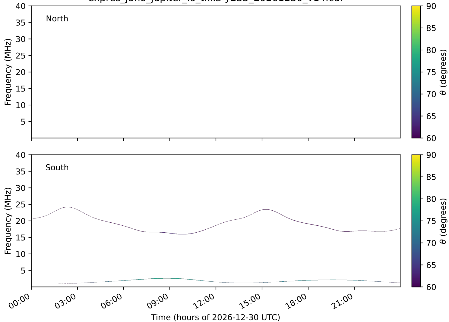
expres_juno_jupiter_io_txka-y235_20261230_v14.cdf
