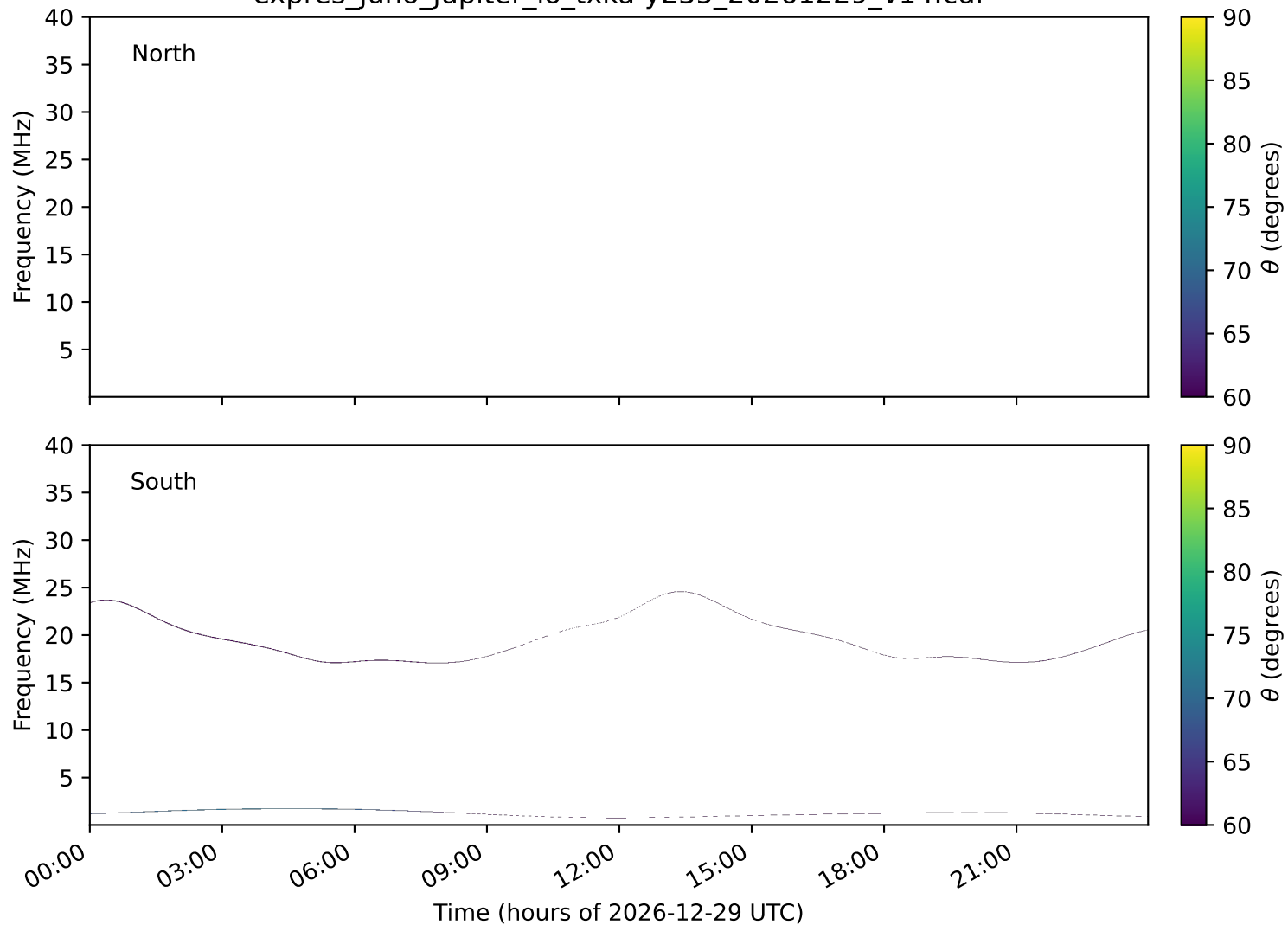
expres_juno_jupiter_io_txka-y235_20261229_v14.cdf
