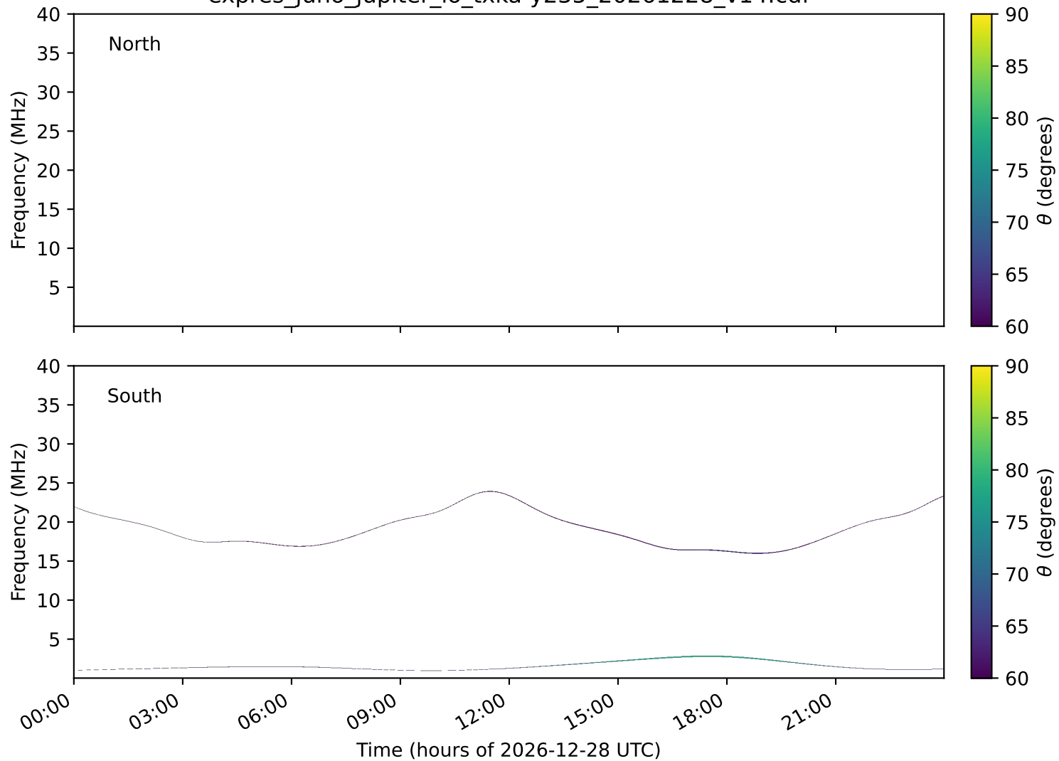
expres_juno_jupiter_io_txka-y235_20261228_v14.cdf
