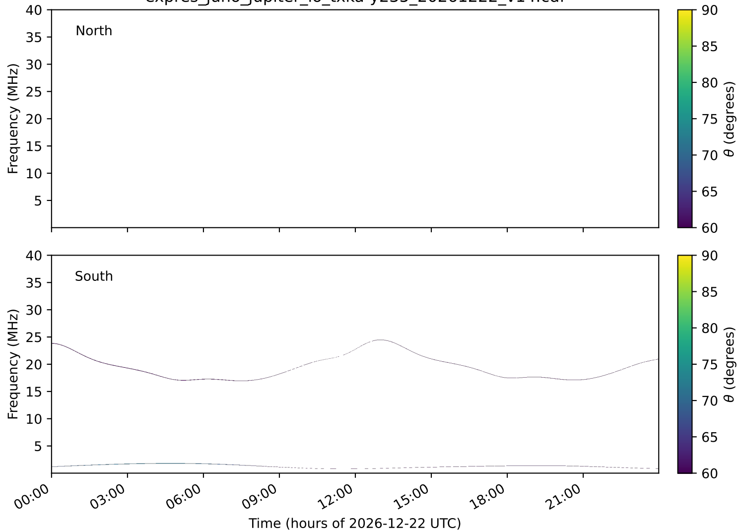
expres_juno_jupiter_io_txka-y235_20261222_v14.cdf
