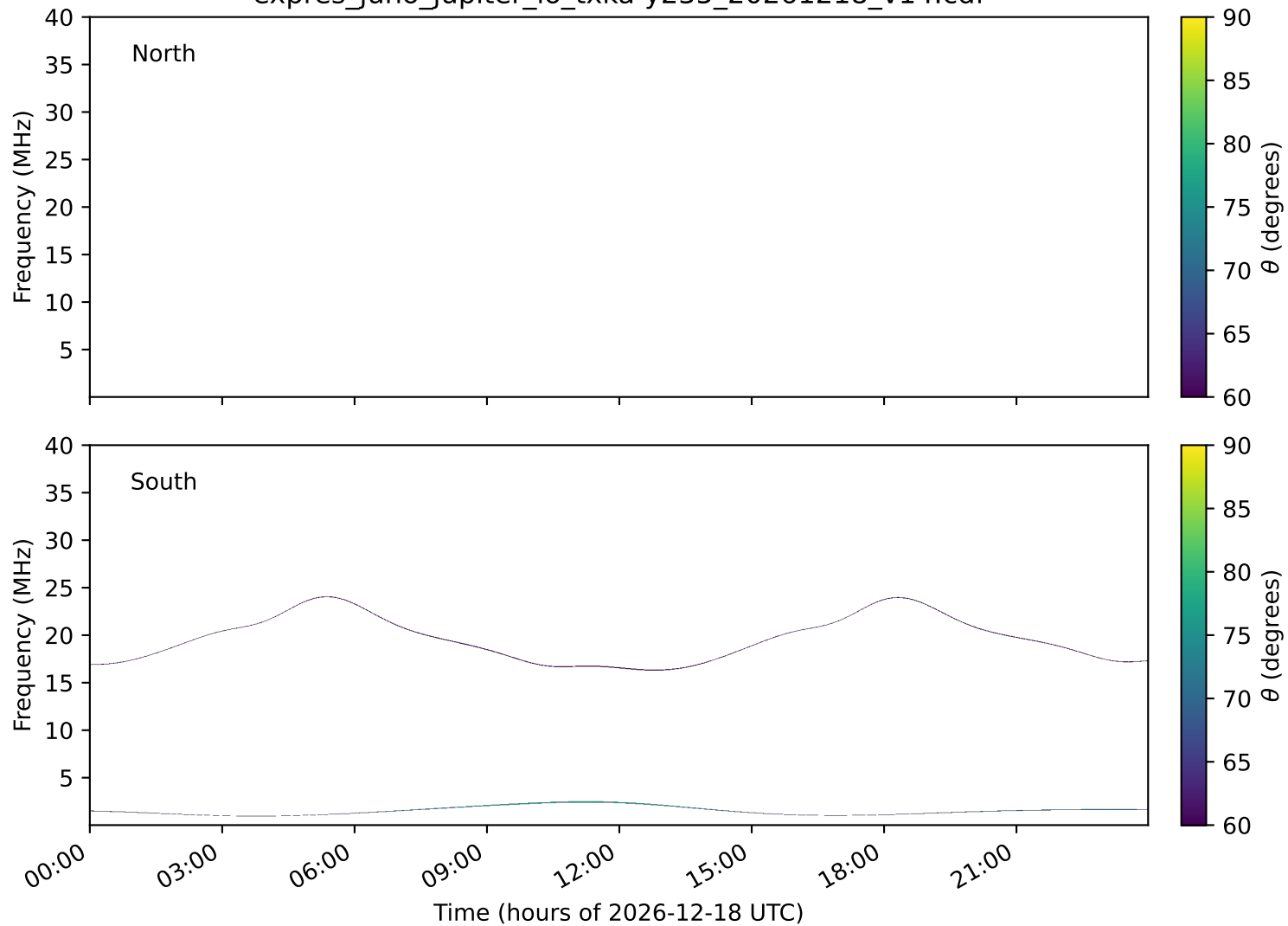
expres_juno_jupiter_io_txka-y235_20261218_v14.cdf
