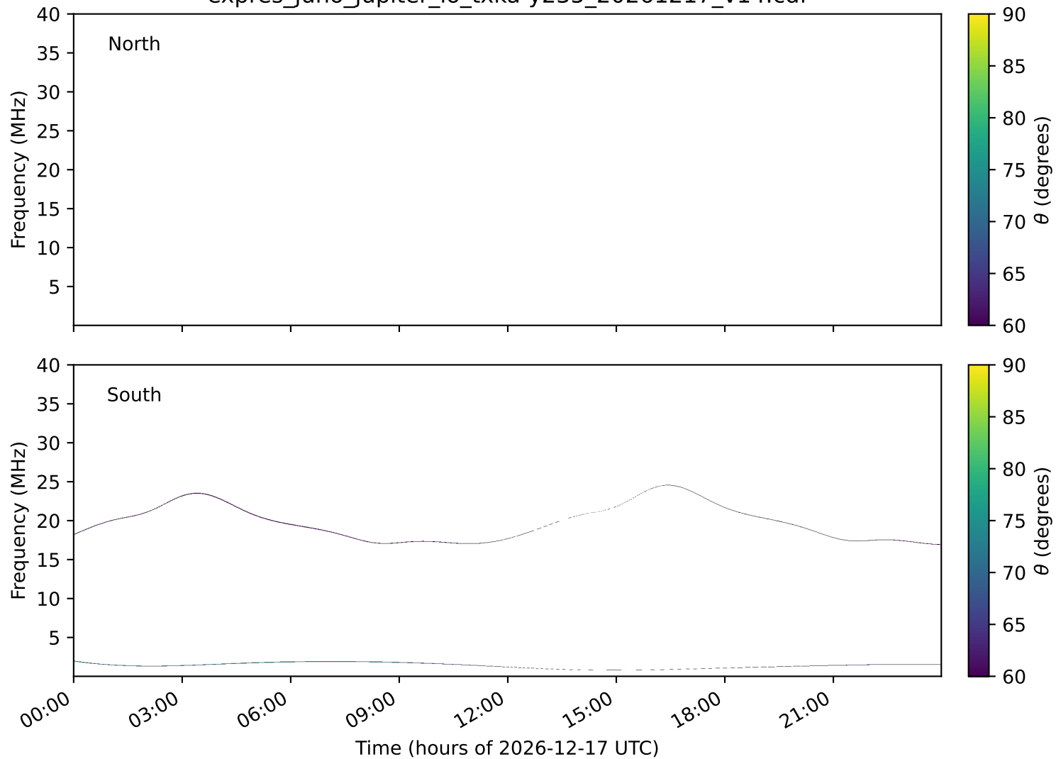
expres_juno_jupiter_io_txka-y235_20261217_v14.cdf
