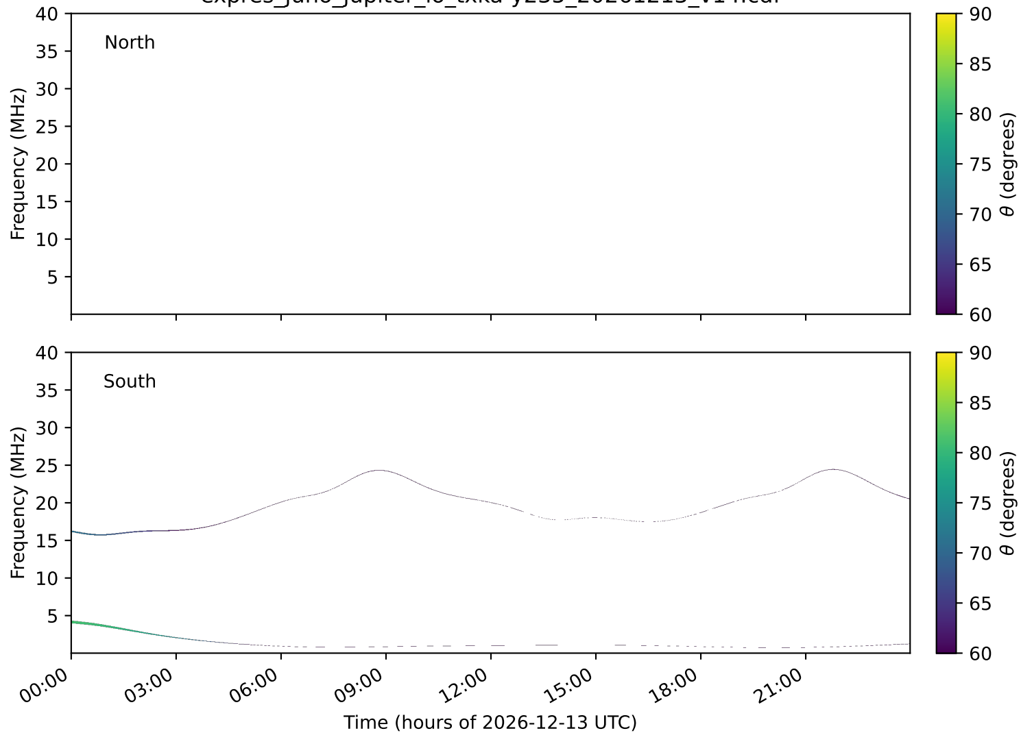
expres_juno_jupiter_io_txka-y235_20261213_v14.cdf
