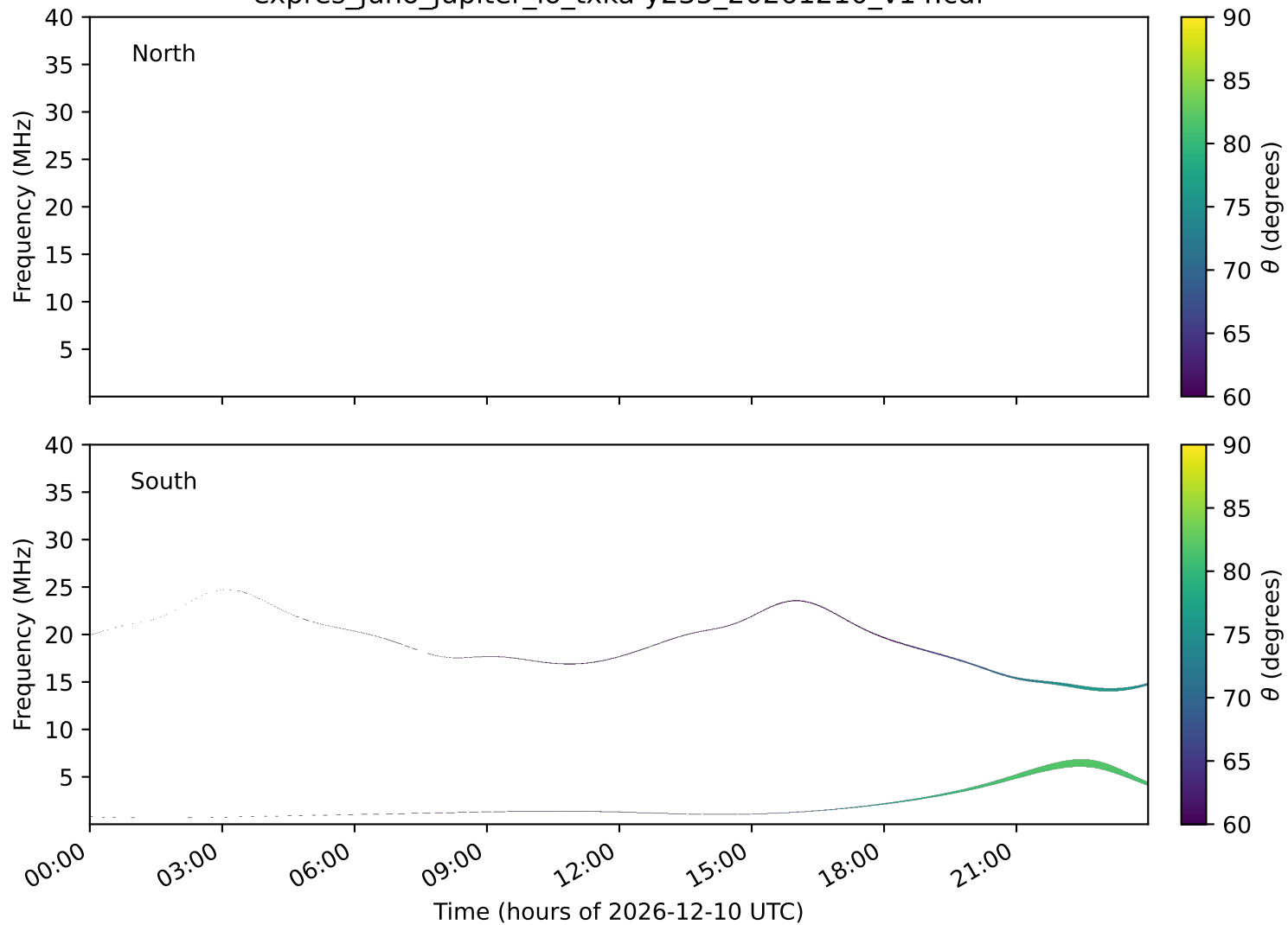
expres_juno_jupiter_io_txka-y235_20261210_v14.cdf
