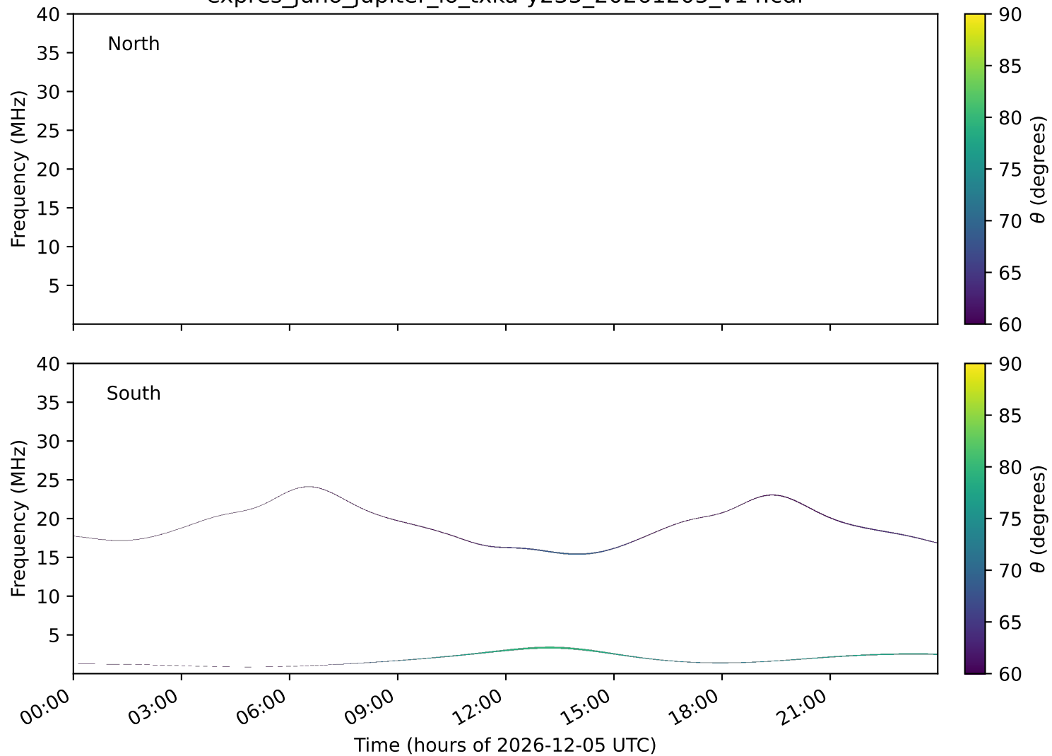
expres_juno_jupiter_io_txka-y235_20261205_v14.cdf
