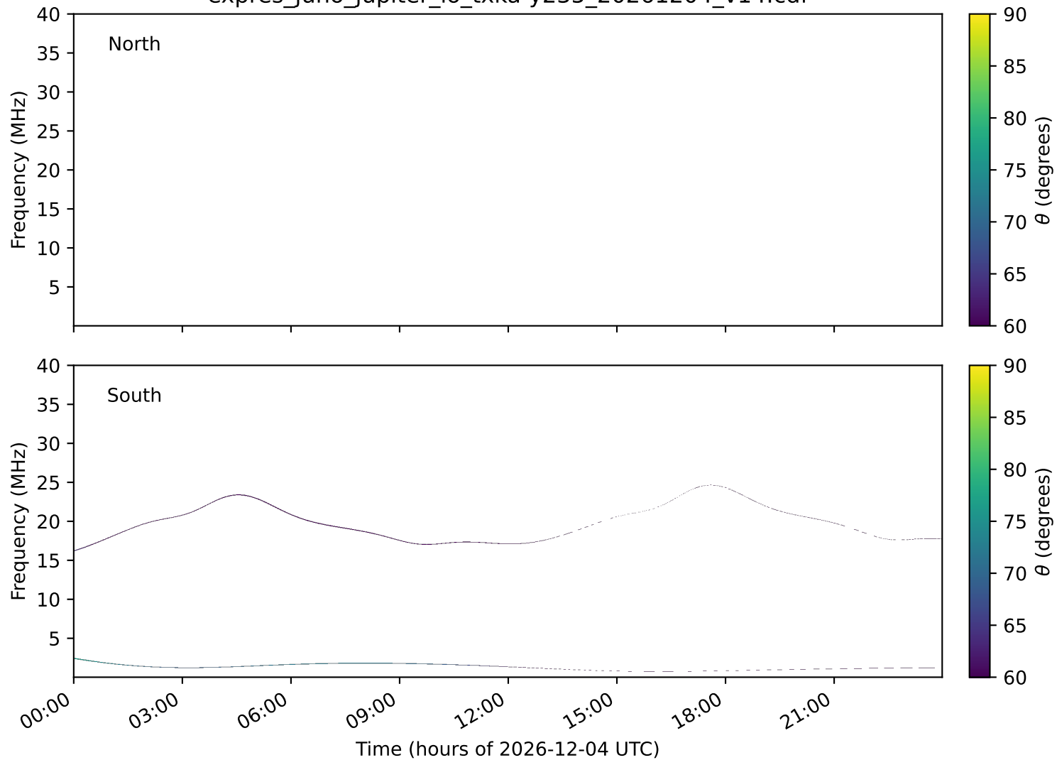
expres_juno_jupiter_io_txka-y235_20261204_v14.cdf
