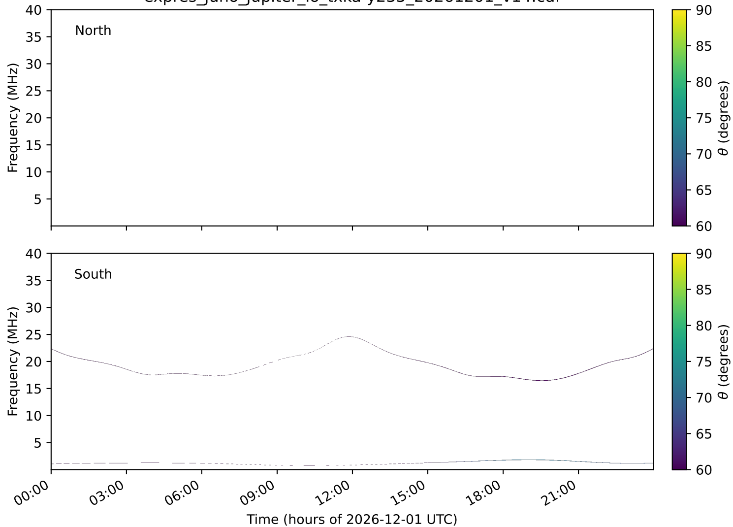
expres_juno_jupiter_io_txka-y235_20261201_v14.cdf
