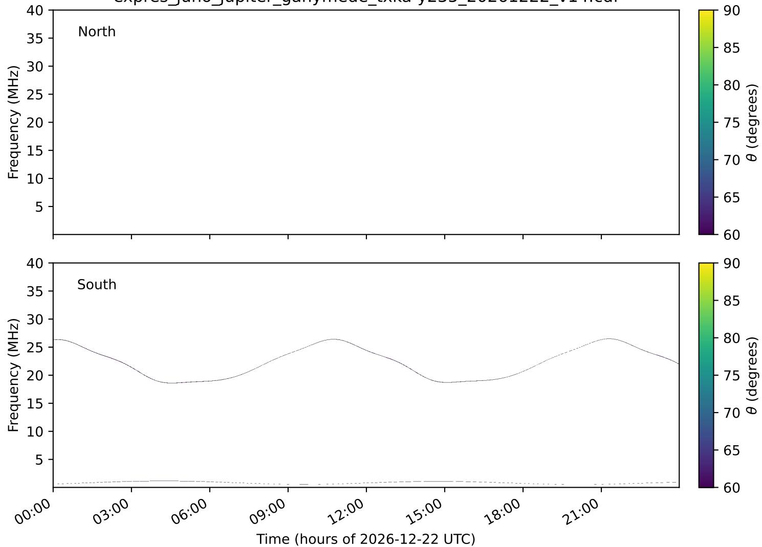
expres_juno_jupiter_ganymede_txka-y235_20261222_v14.cdf
