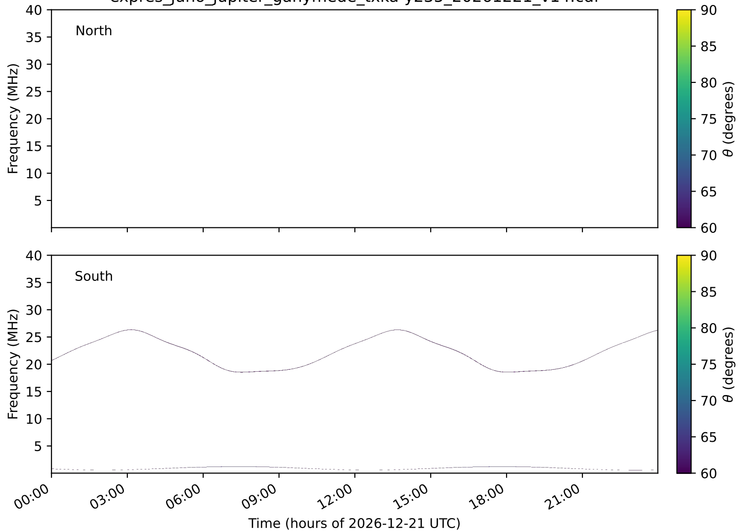
expres_juno_jupiter_ganymede_txka-y235_20261221_v14.cdf
