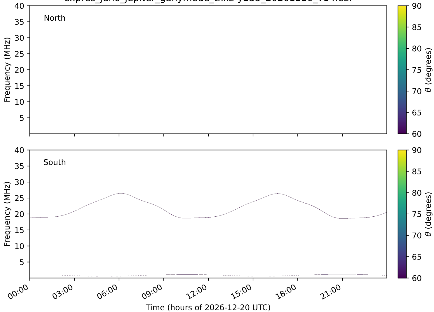
expres_juno_jupiter_ganymede_txka-y235_20261220_v14.cdf
