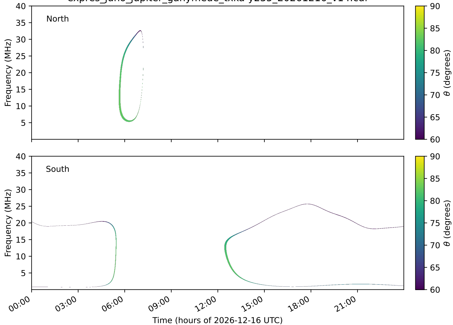
expres_juno_jupiter_ganymede_txka-y235_20261216_v14.cdf
