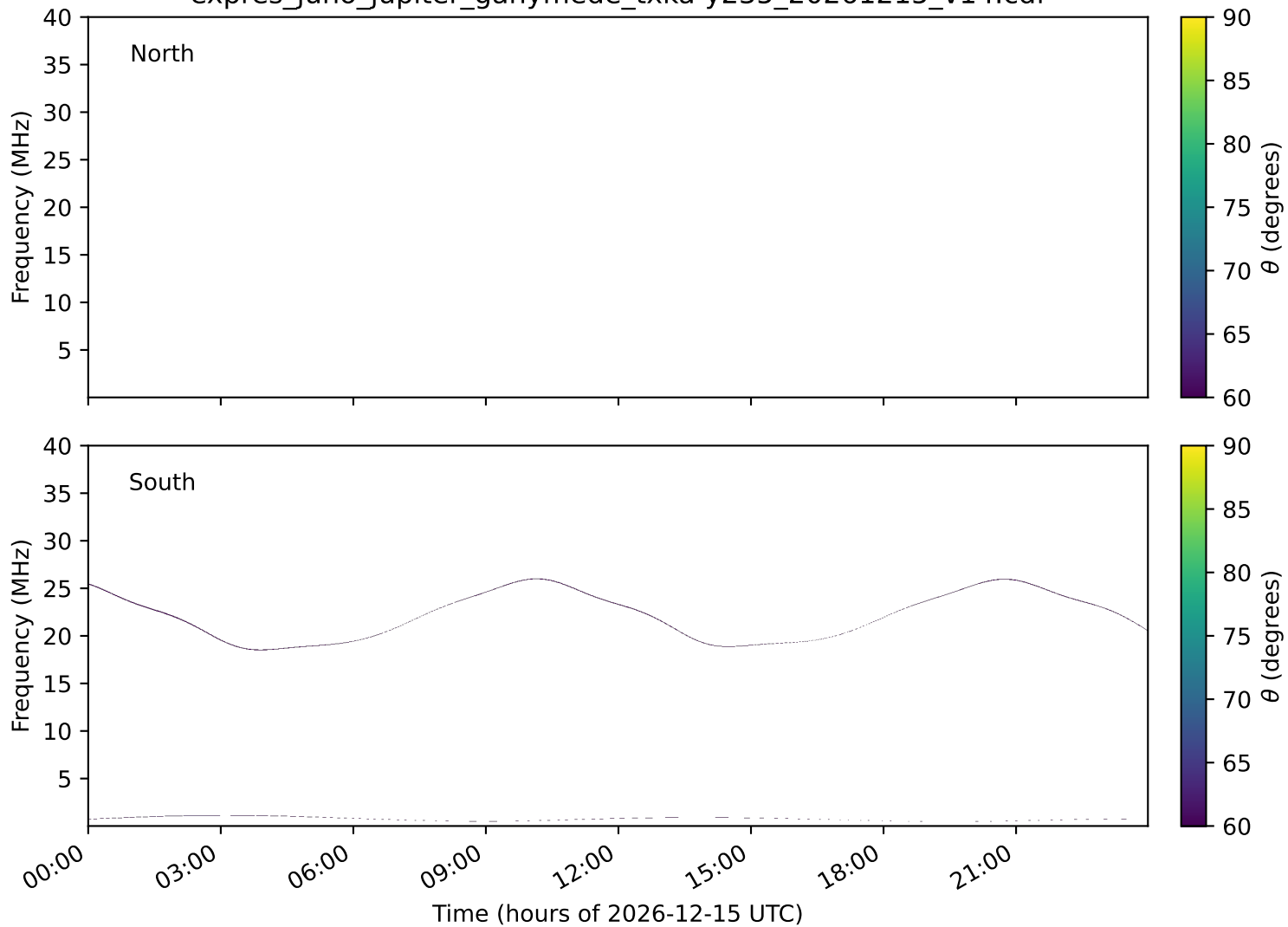
expres_juno_jupiter_ganymede_txka-y235_20261215_v14.cdf
