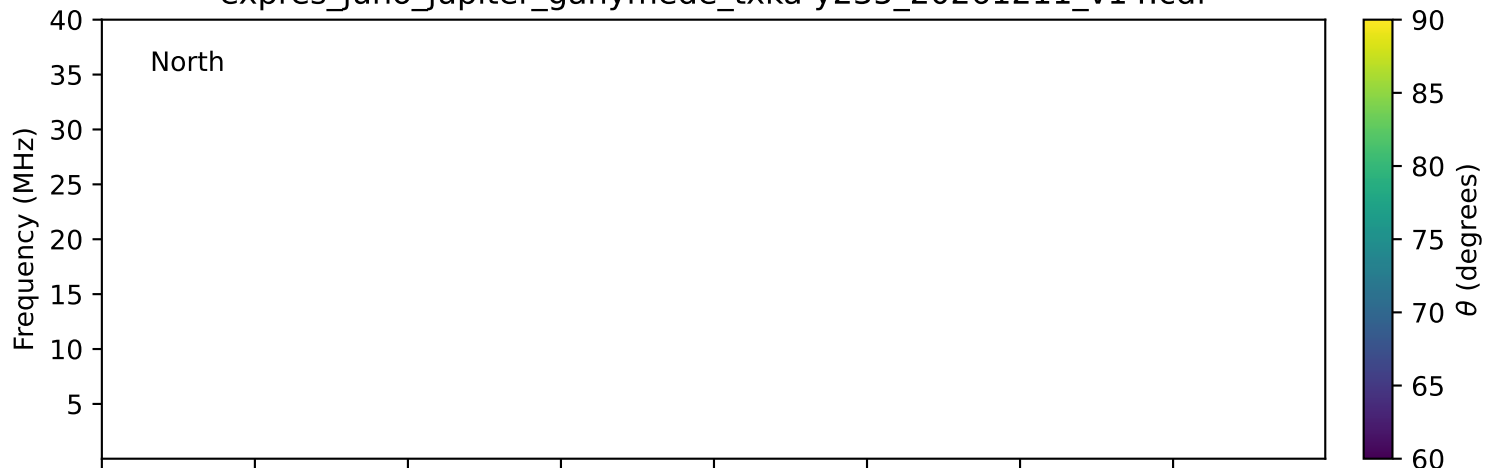
expres_juno_jupiter_ganymede_txka-y235_20261211_v14.cdf
