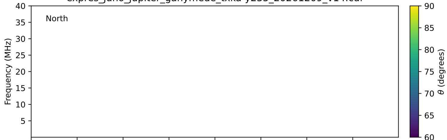
expres_juno_jupiter_ganymede_txka-y235_20261209_v14.cdf
