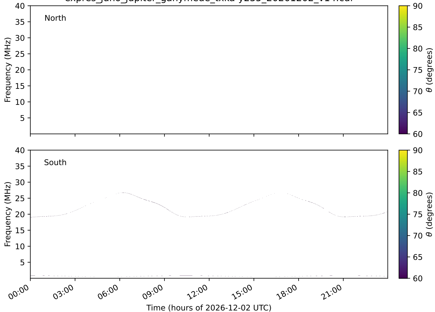
expres_juno_jupiter_ganymede_txka-y235_20261202_v14.cdf
