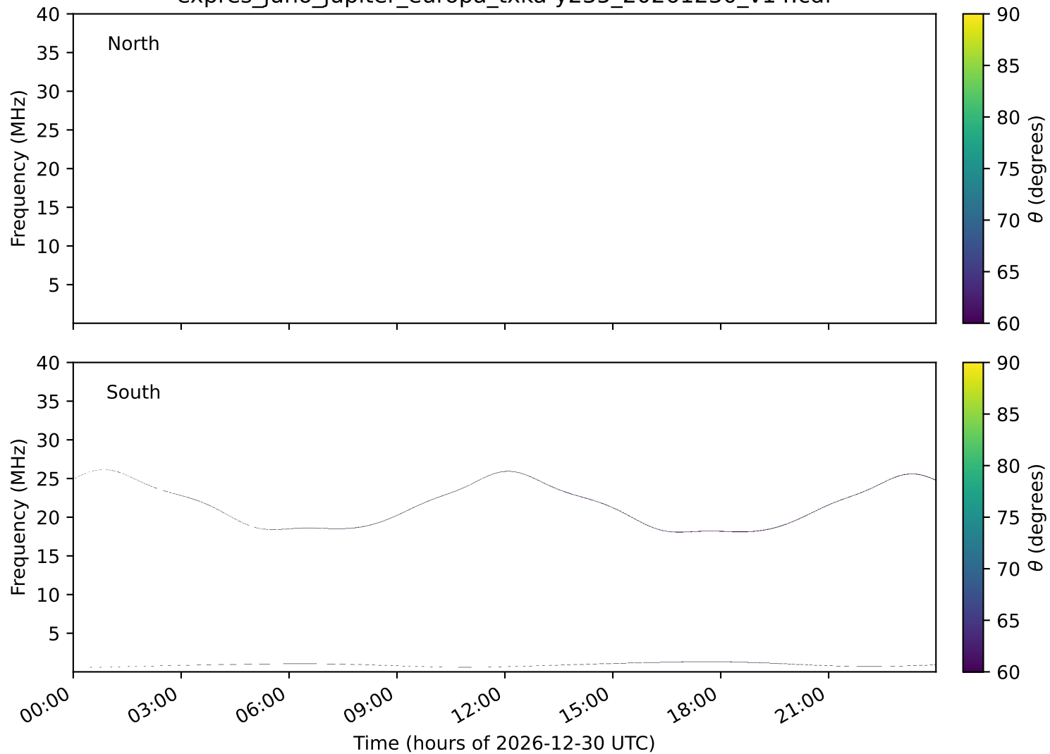
expres_juno_jupiter_europa_txka-y235_20261230_v14.cdf
