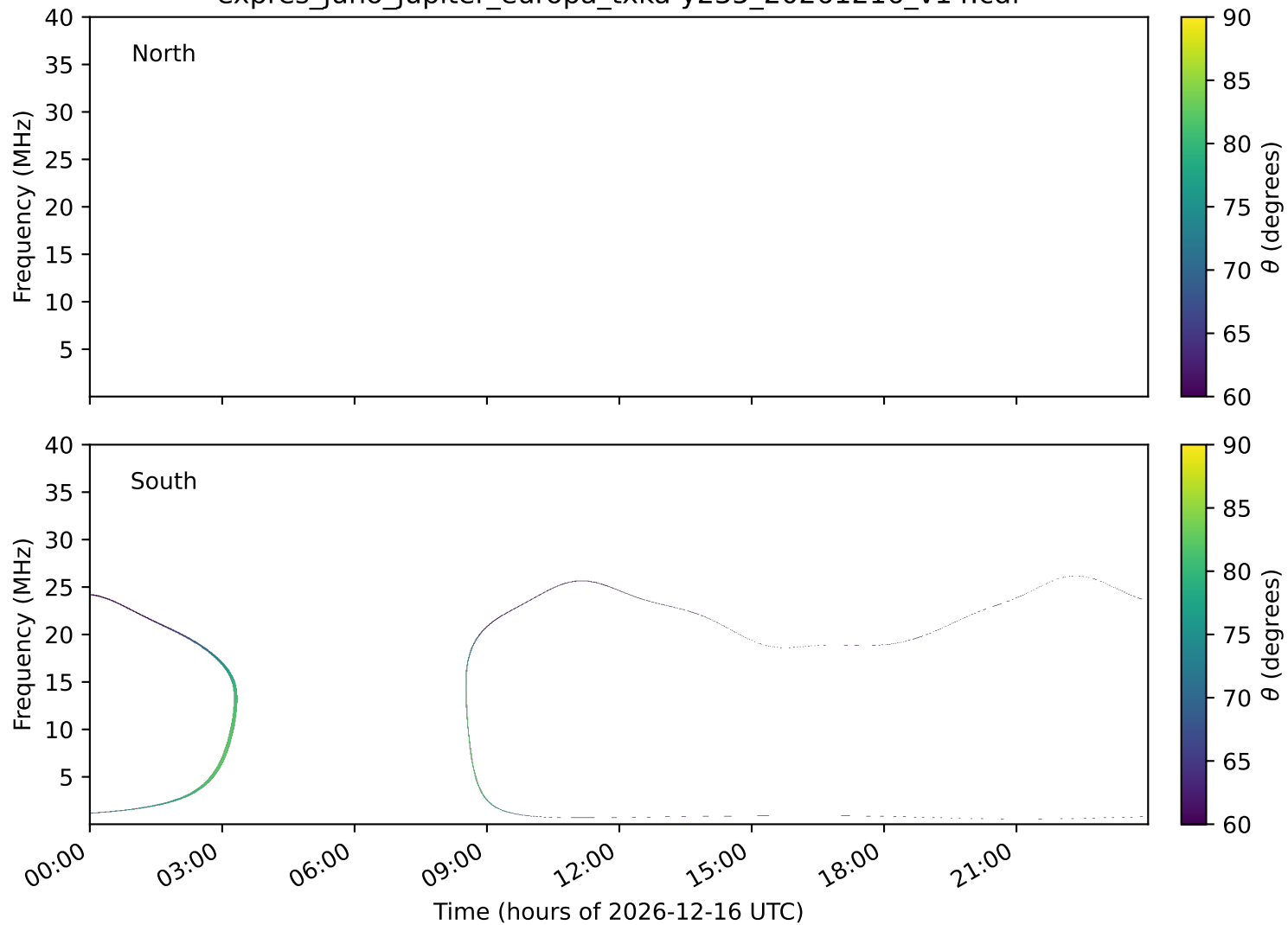
expres_juno_jupiter_europa_txka-y235_20261216_v14.cdf
