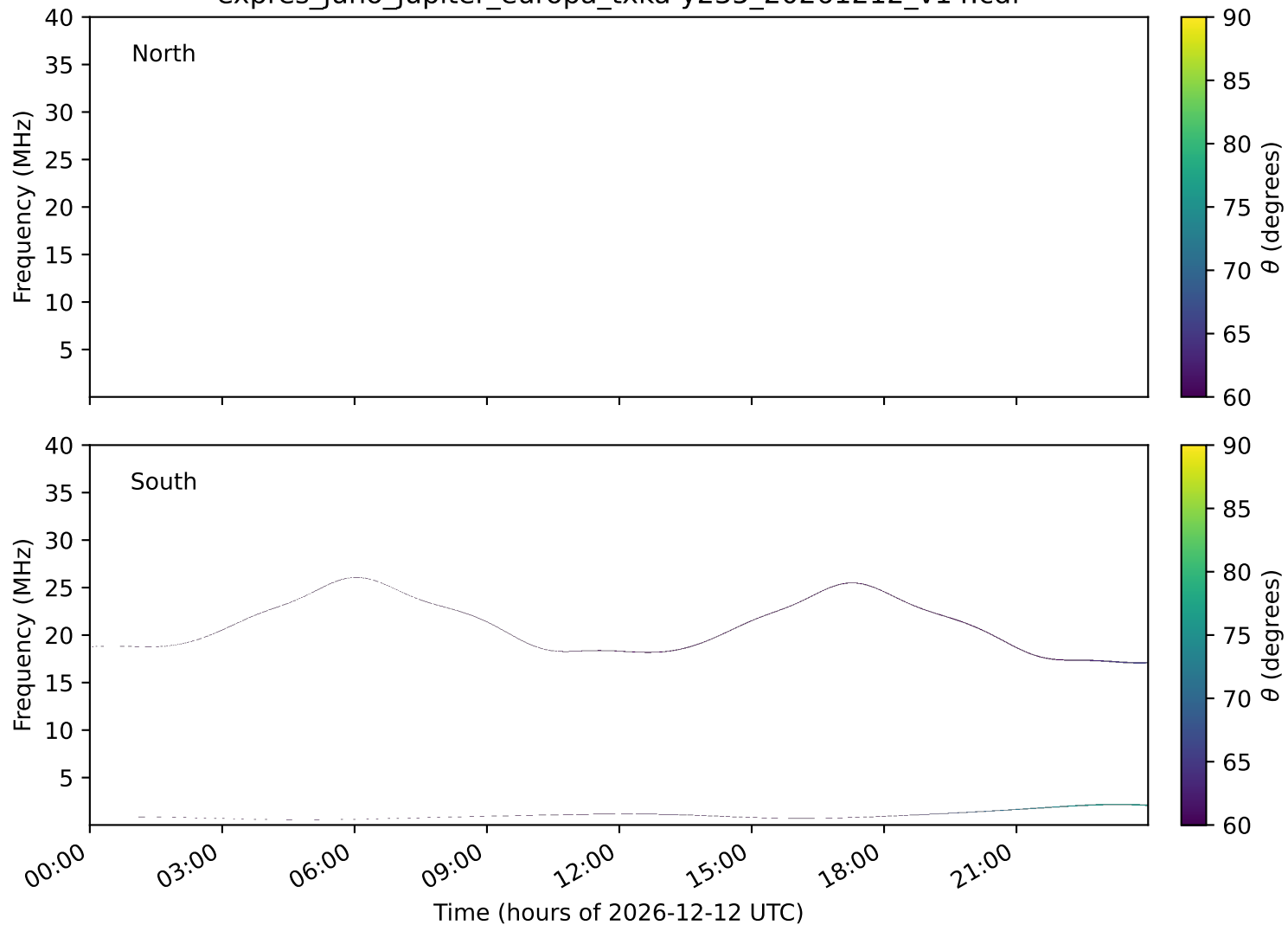
expres_juno_jupiter_europa_txka-y235_20261212_v14.cdf
