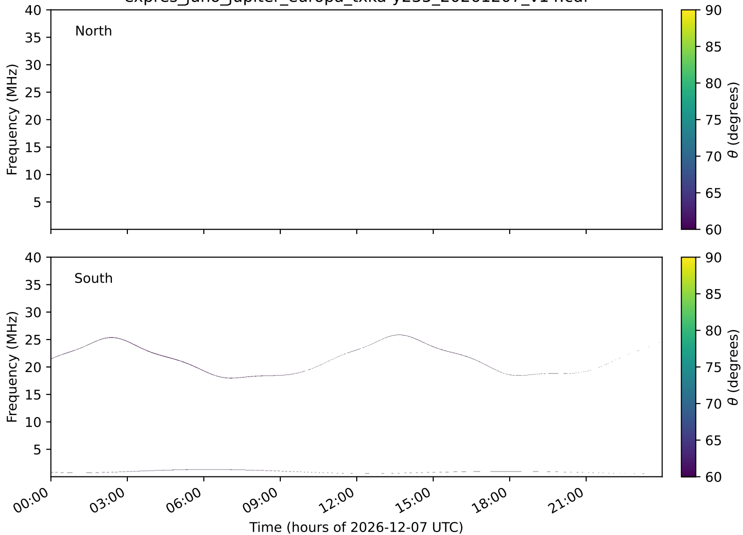
expres_juno_jupiter_europa_txka-y235_20261207_v14.cdf
