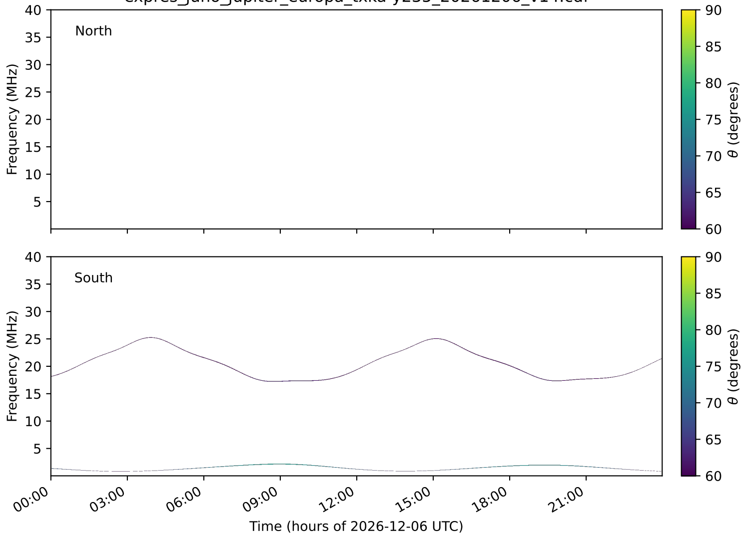
expres_juno_jupiter_europa_txka-y235_20261206_v14.cdf
