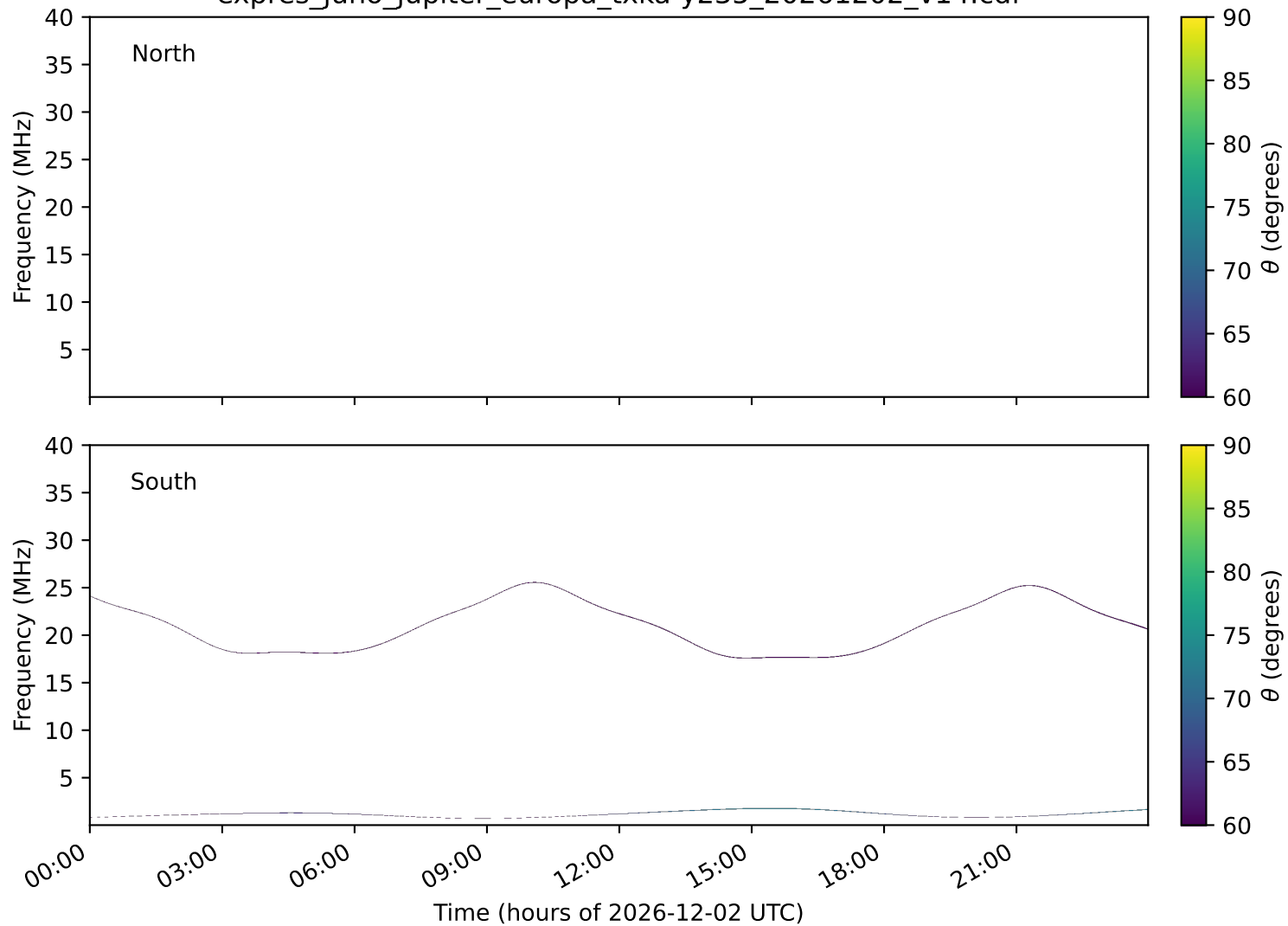
expres_juno_jupiter_europa_txka-y235_20261202_v14.cdf
