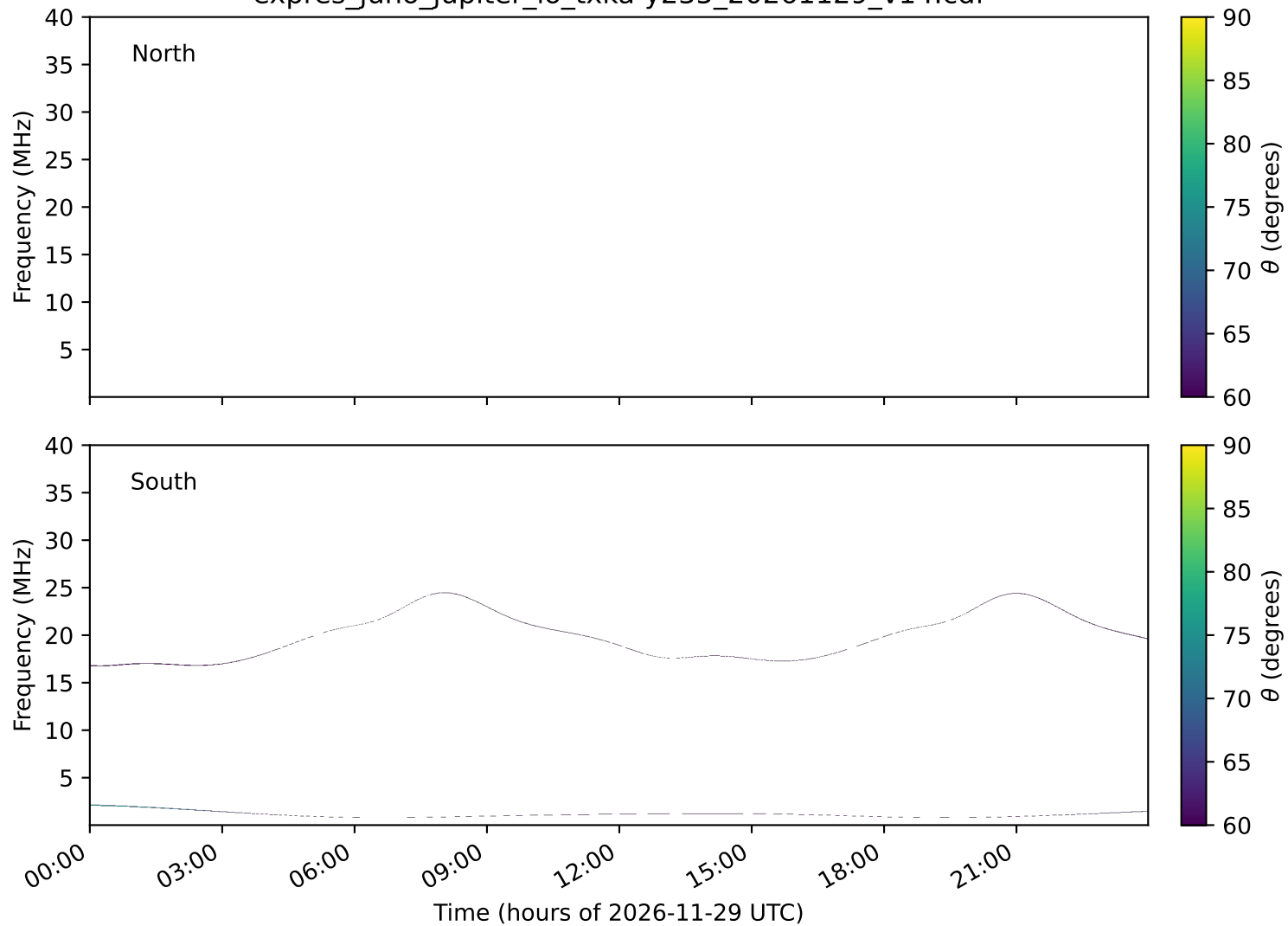
expres_juno_jupiter_io_txka-y235_20261129_v14.cdf
