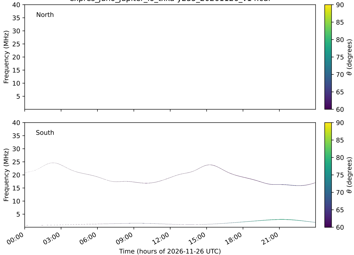
expres_juno_jupiter_io_txka-y235_20261126_v14.cdf
