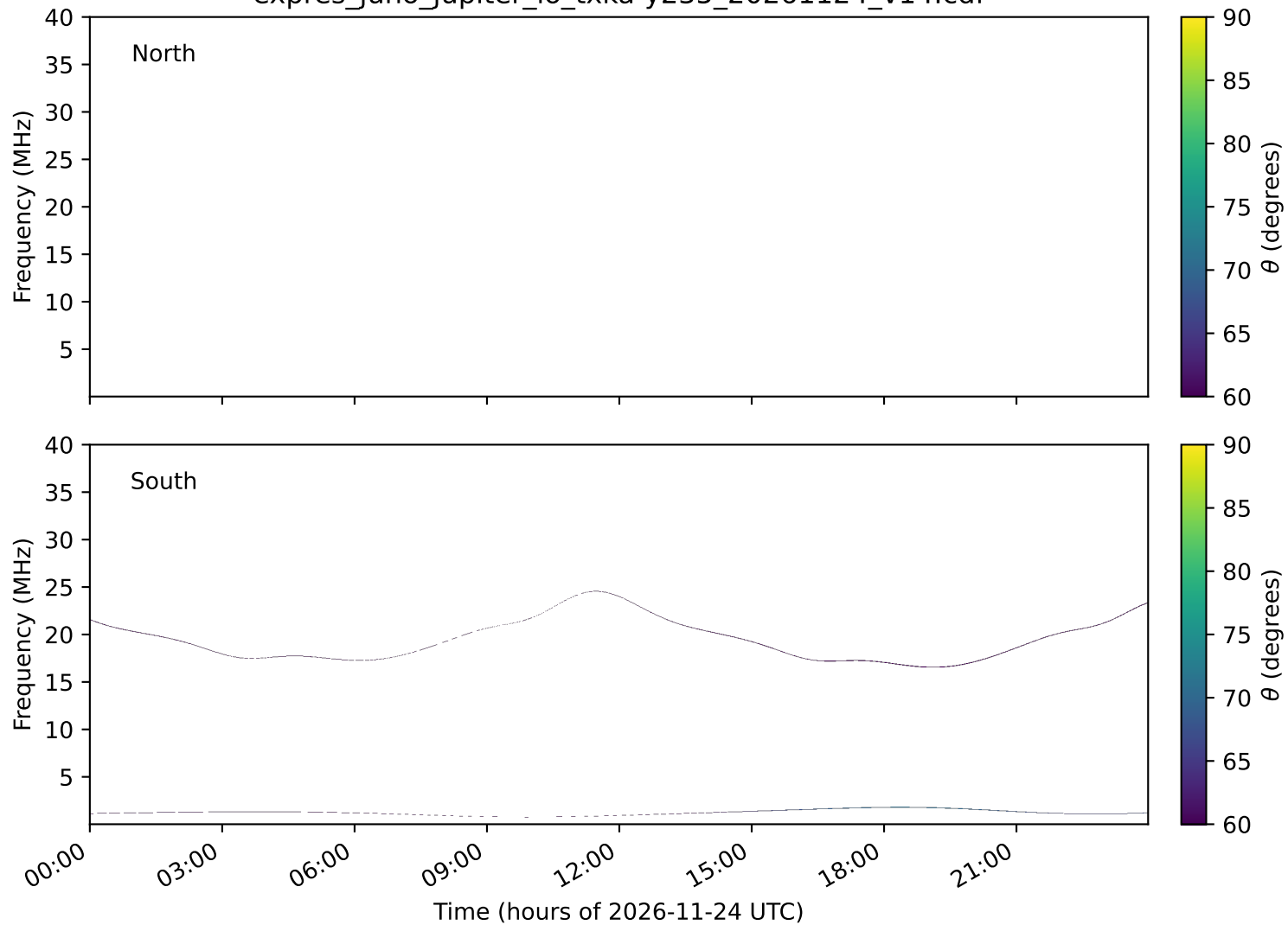
expres_juno_jupiter_io_txka-y235_20261124_v14.cdf
