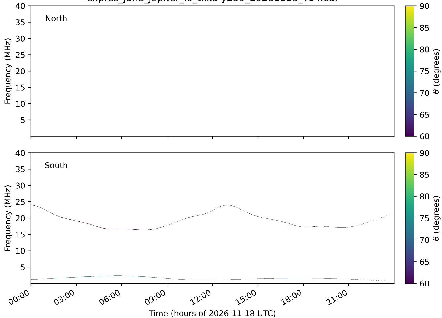
expres_juno_jupiter_io_txka-y235_20261118_v14.cdf
