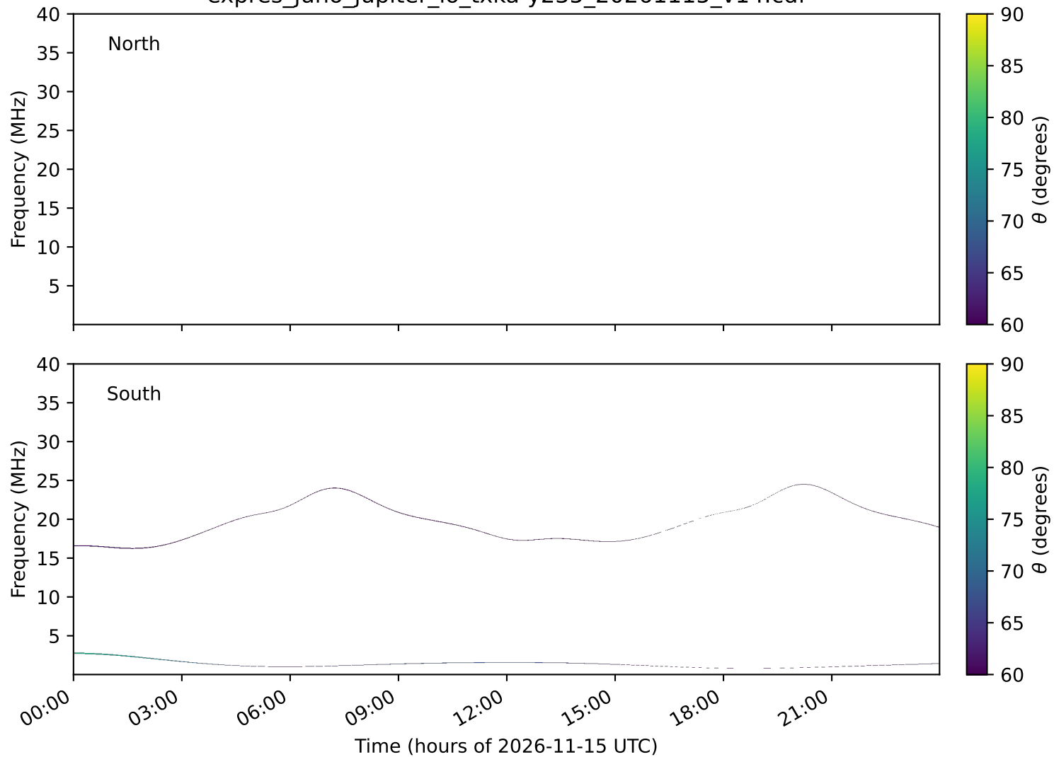
expres_juno_jupiter_io_txka-y235_20261115_v14.cdf
