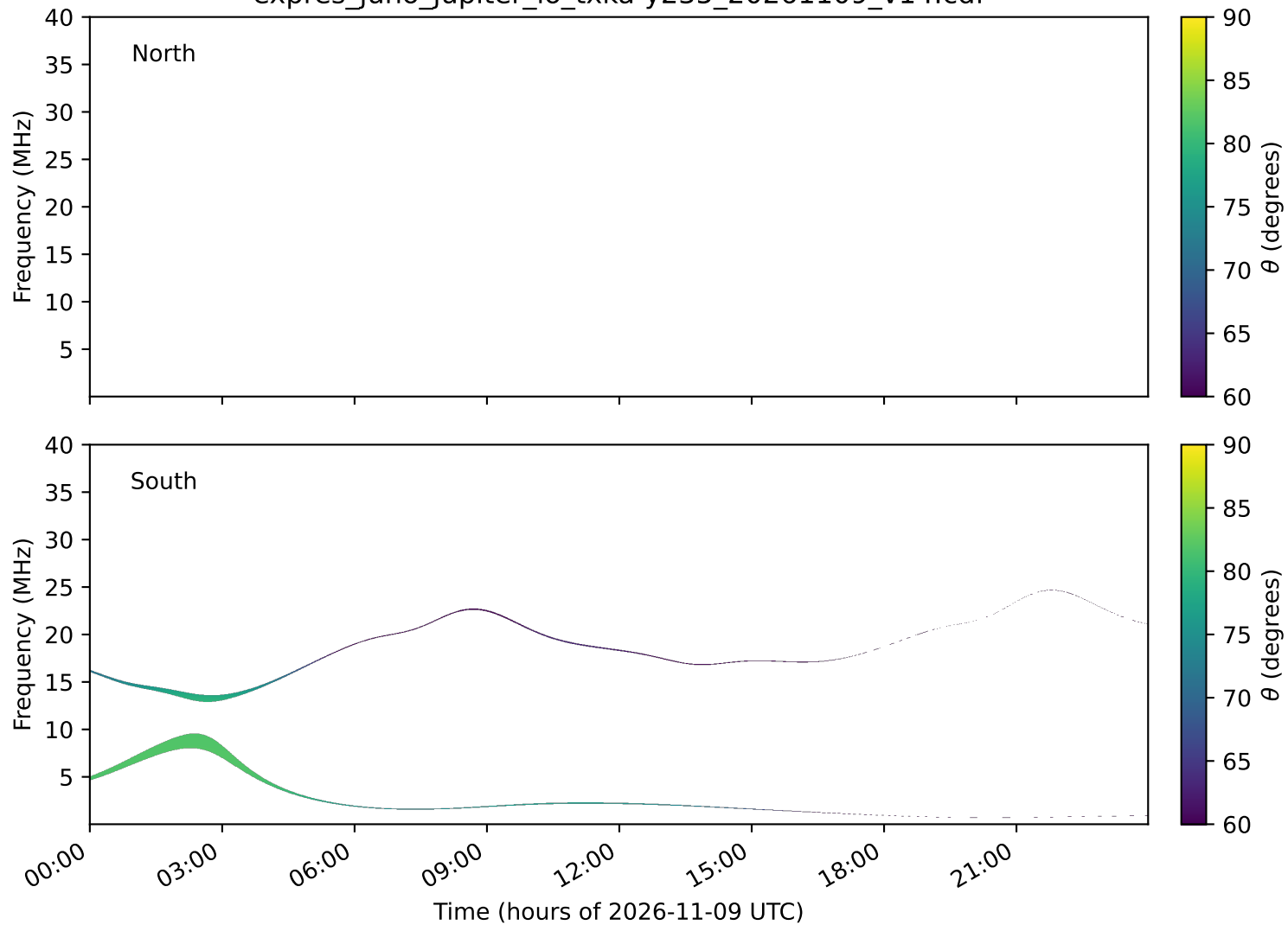
expres_juno_jupiter_io_txka-y235_20261109_v14.cdf
