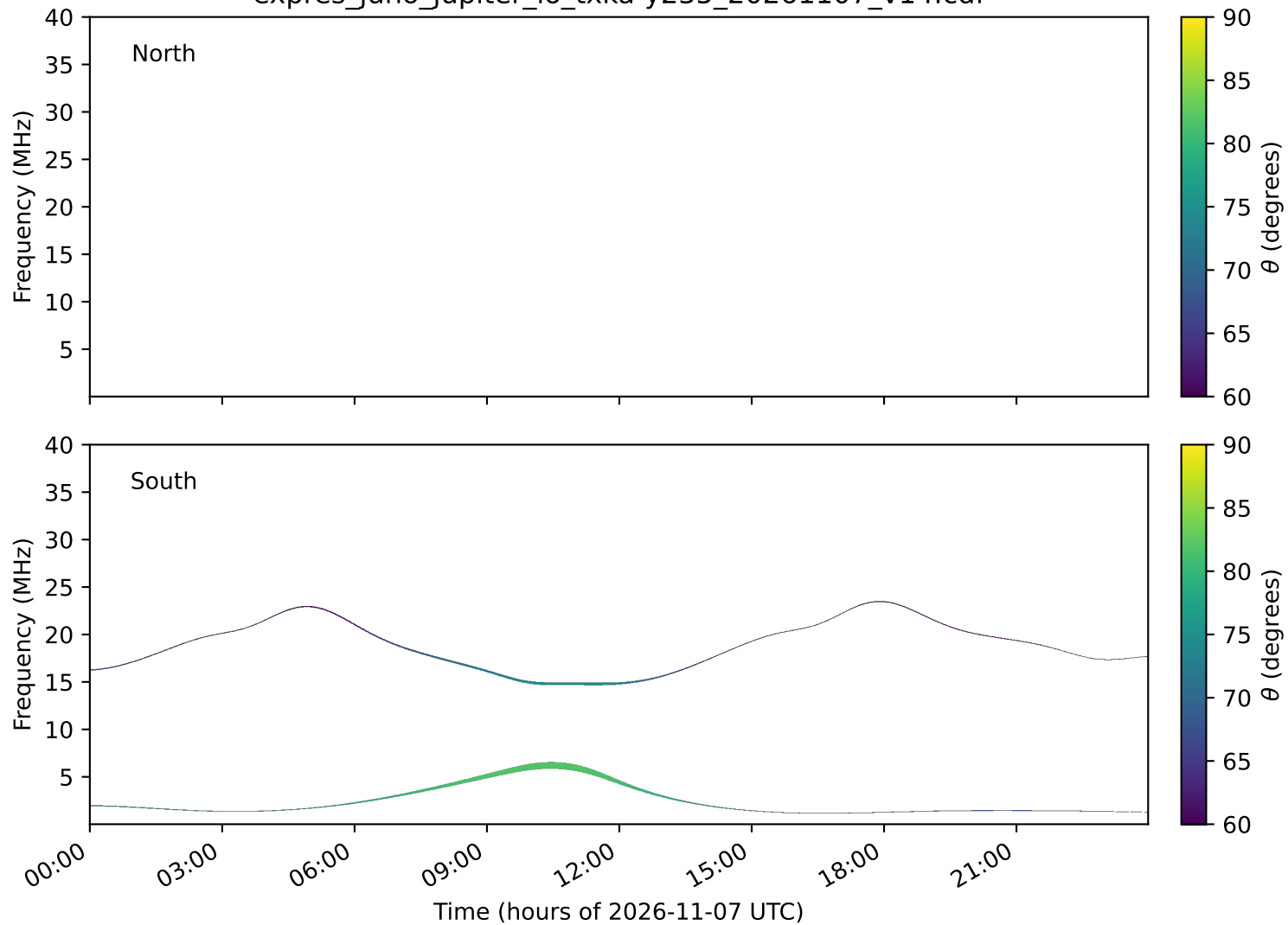
expres_juno_jupiter_io_txka-y235_20261107_v14.cdf
