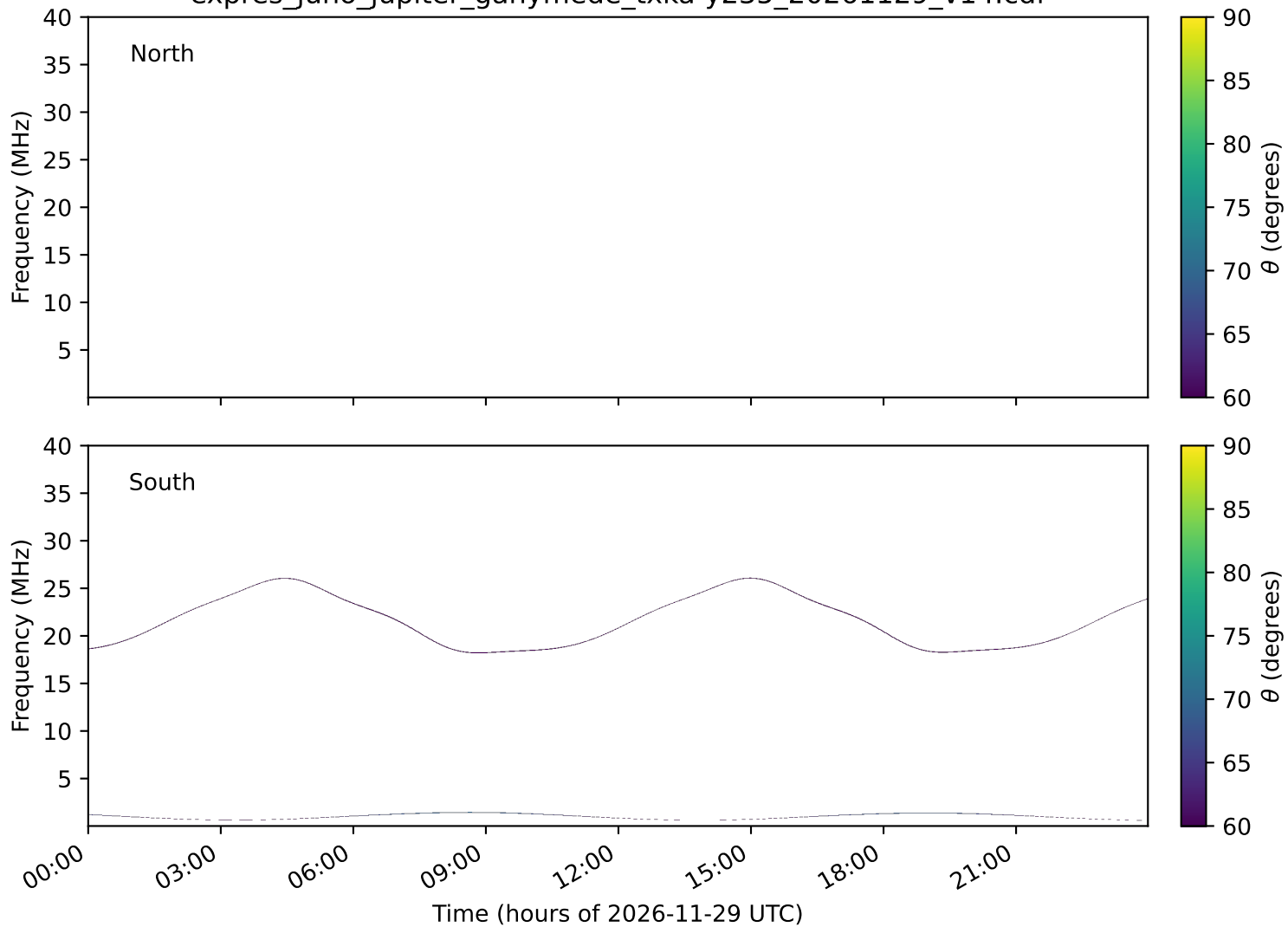
expres_juno_jupiter_ganymede_txka-y235_20261129_v14.cdf
