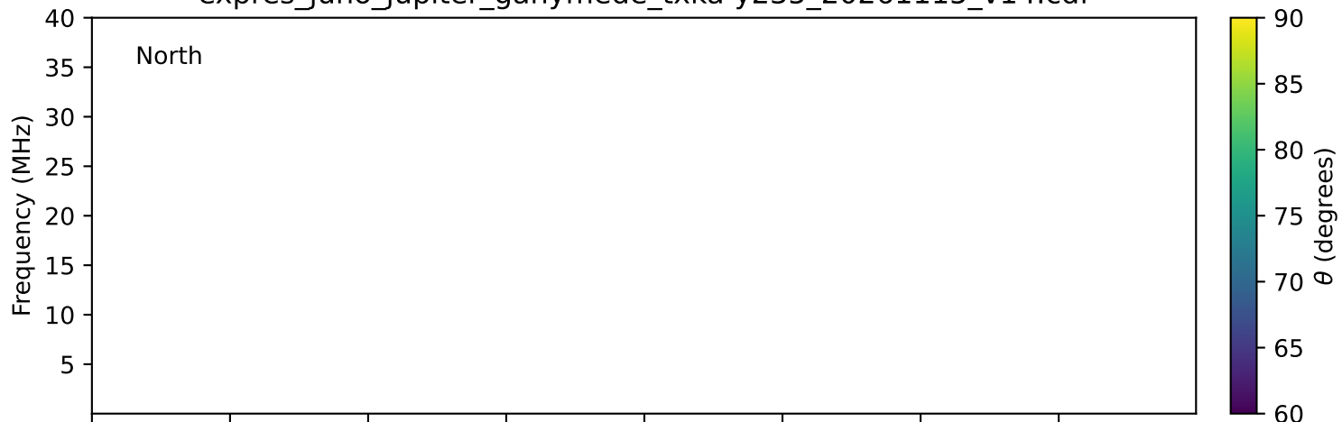
expres_juno_jupiter_ganymede_txka-y235_20261115_v14.cdf
