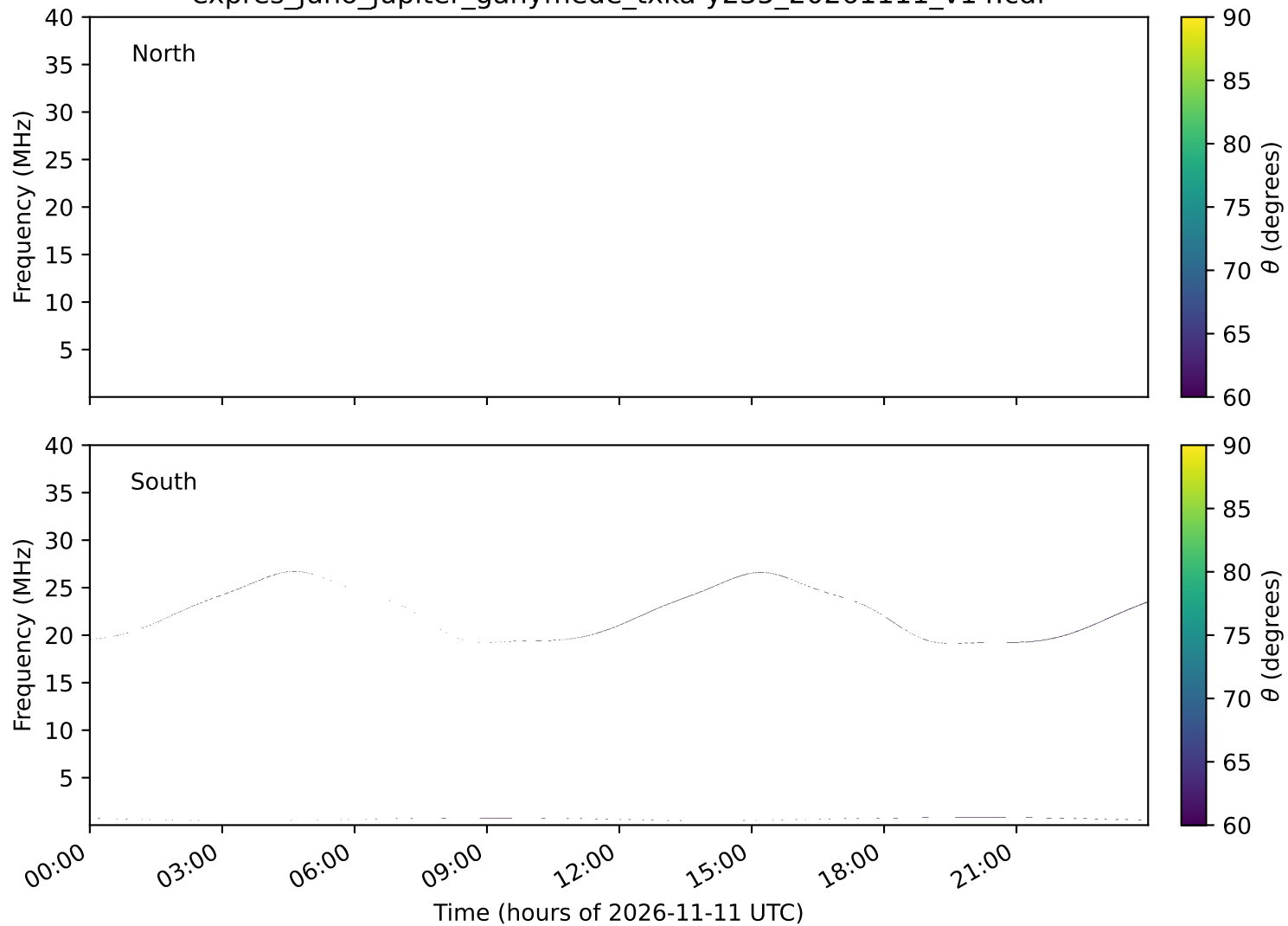
expres_juno_jupiter_ganymede_txka-y235_20261111_v14.cdf
