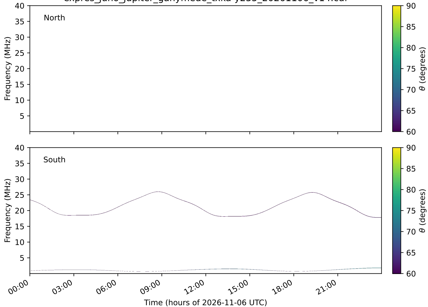
expres_juno_jupiter_ganymede_txka-y235_20261106_v14.cdf
