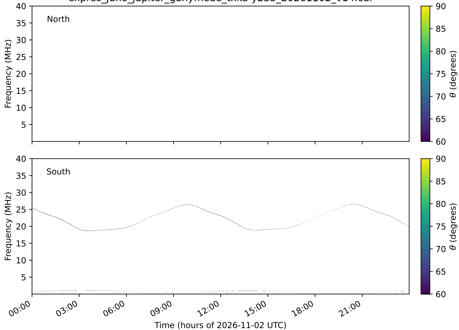
expres_juno_jupiter_ganymede_txka-y235_20261102_v14.cdf
