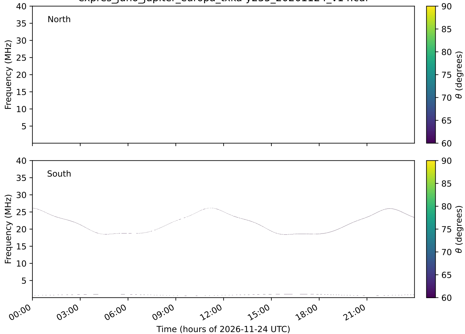
expres_juno_jupiter_europa_txka-y235_20261124_v14.cdf
