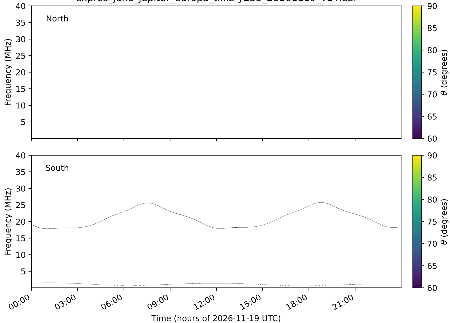
expres_juno_jupiter_europa_txka-y235_20261119_v14.cdf
