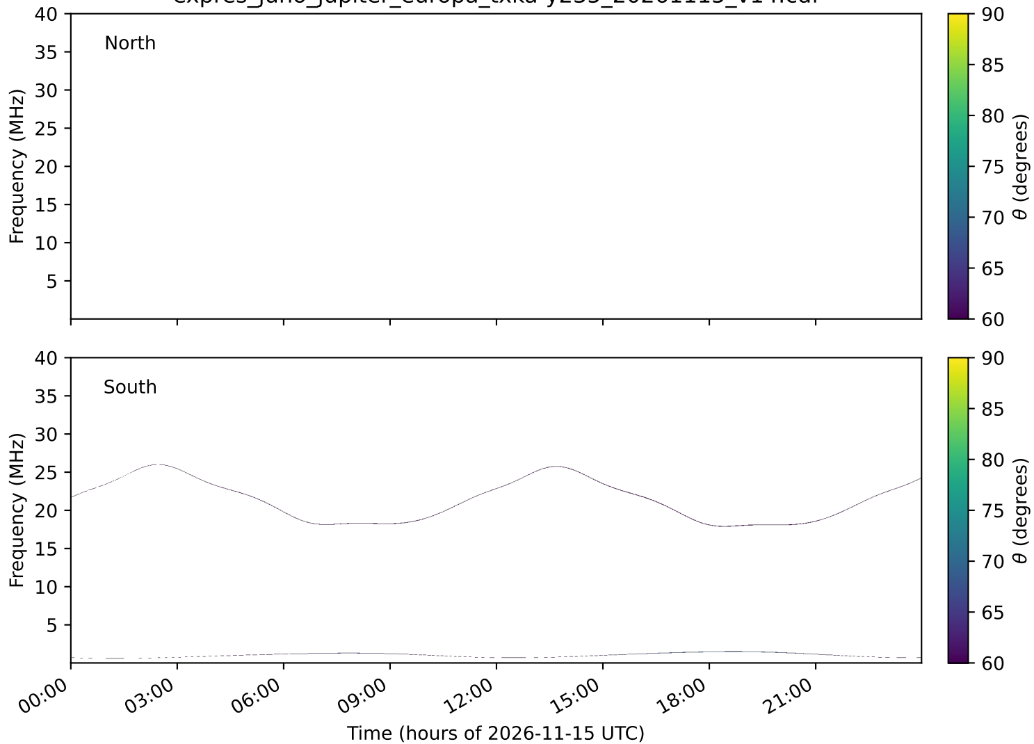
expres_juno_jupiter_europa_txka-y235_20261115_v14.cdf
