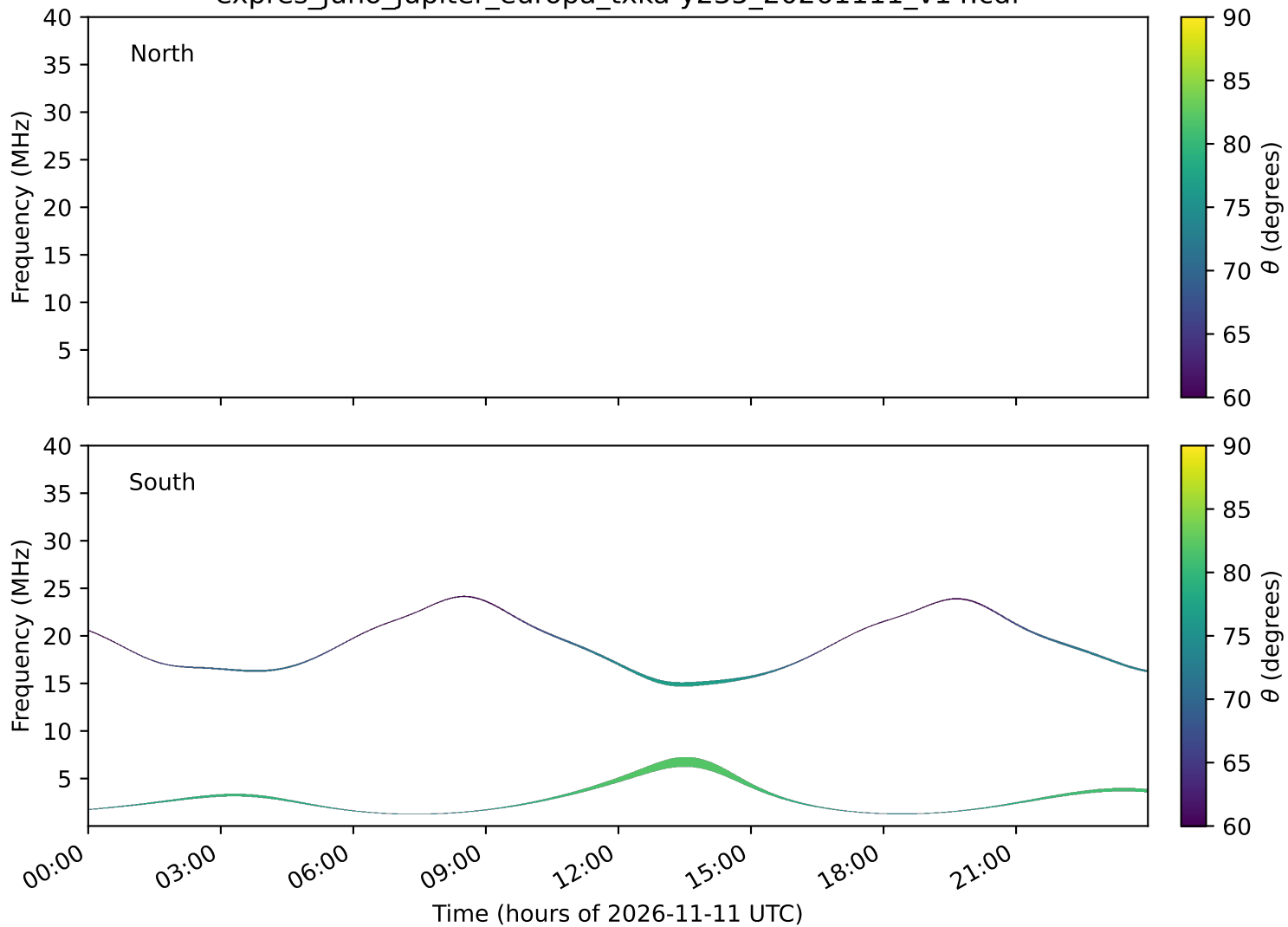
expres_juno_jupiter_europa_txka-y235_20261111_v14.cdf
