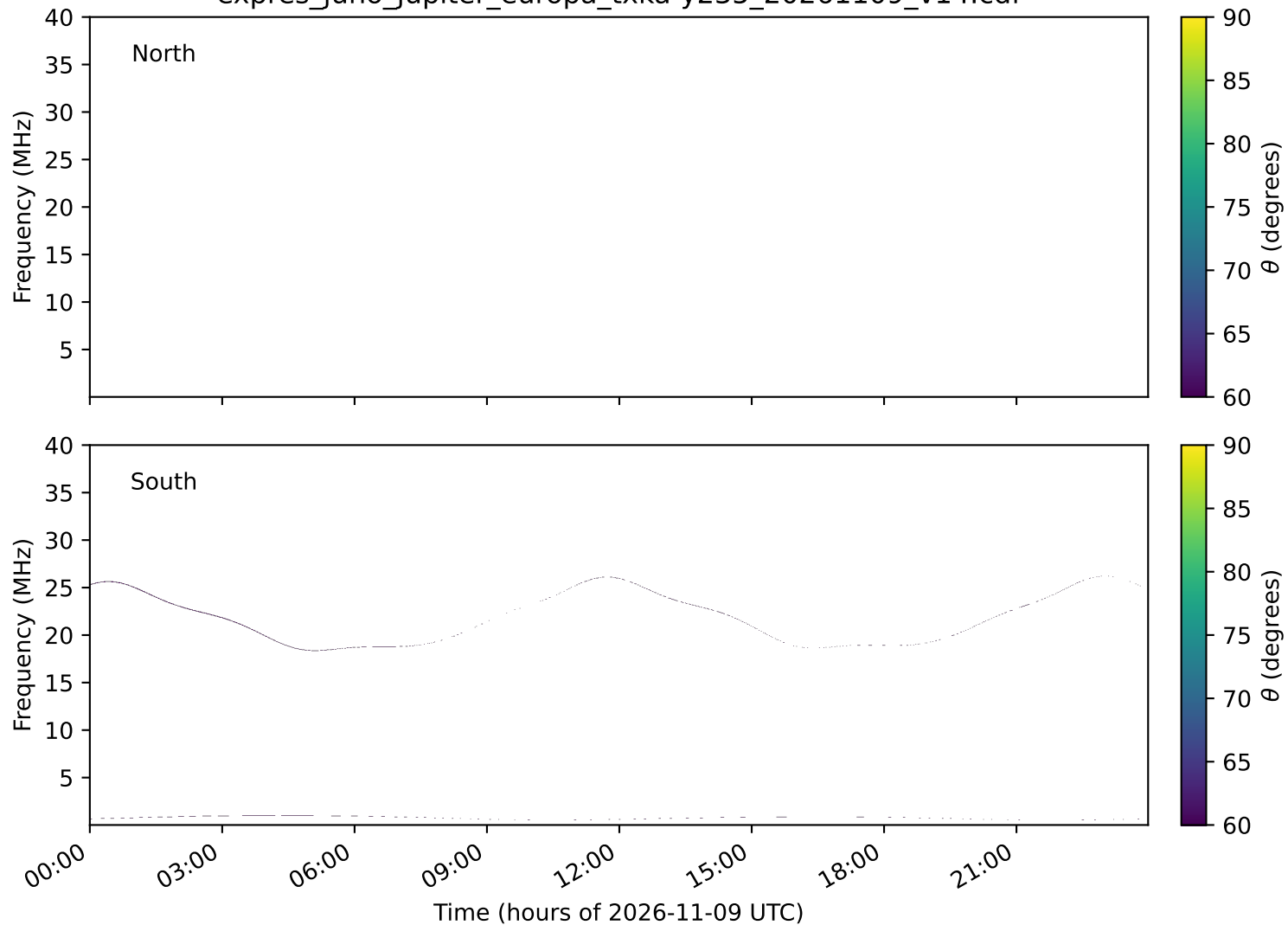
expres_juno_jupiter_europa_txka-y235_20261109_v14.cdf
