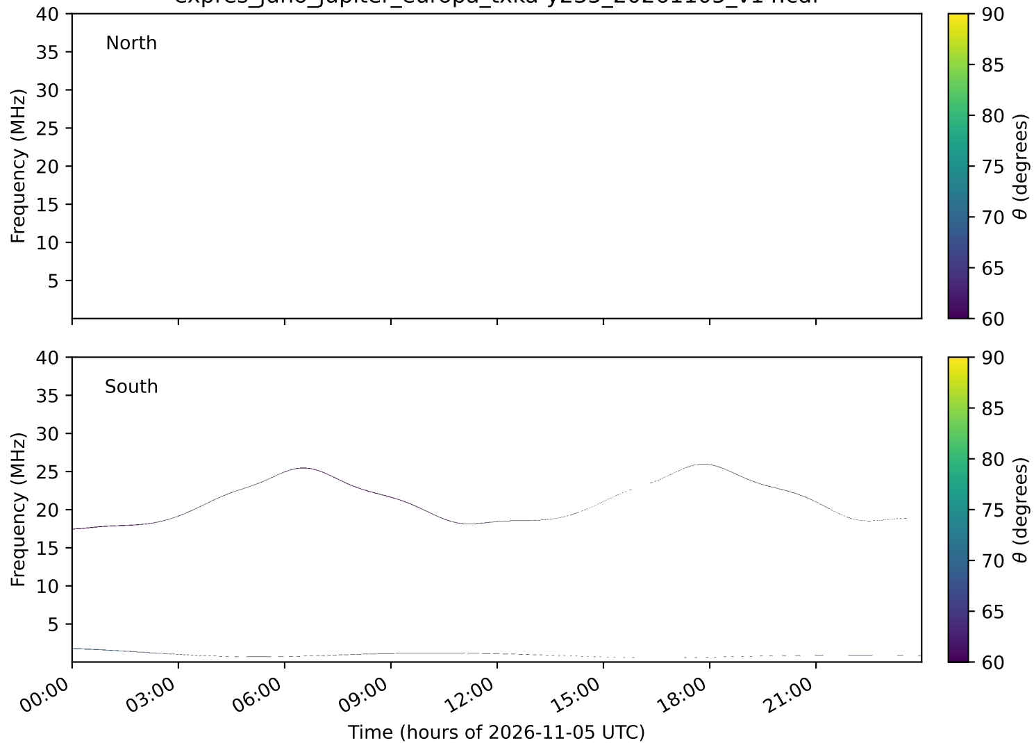
expres_juno_jupiter_europa_txka-y235_20261105_v14.cdf
