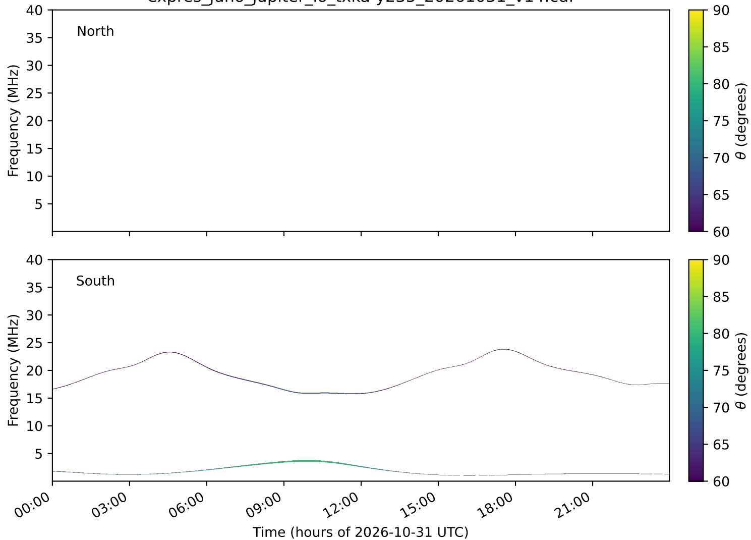
expres_juno_jupiter_io_txka-y235_20261031_v14.cdf
